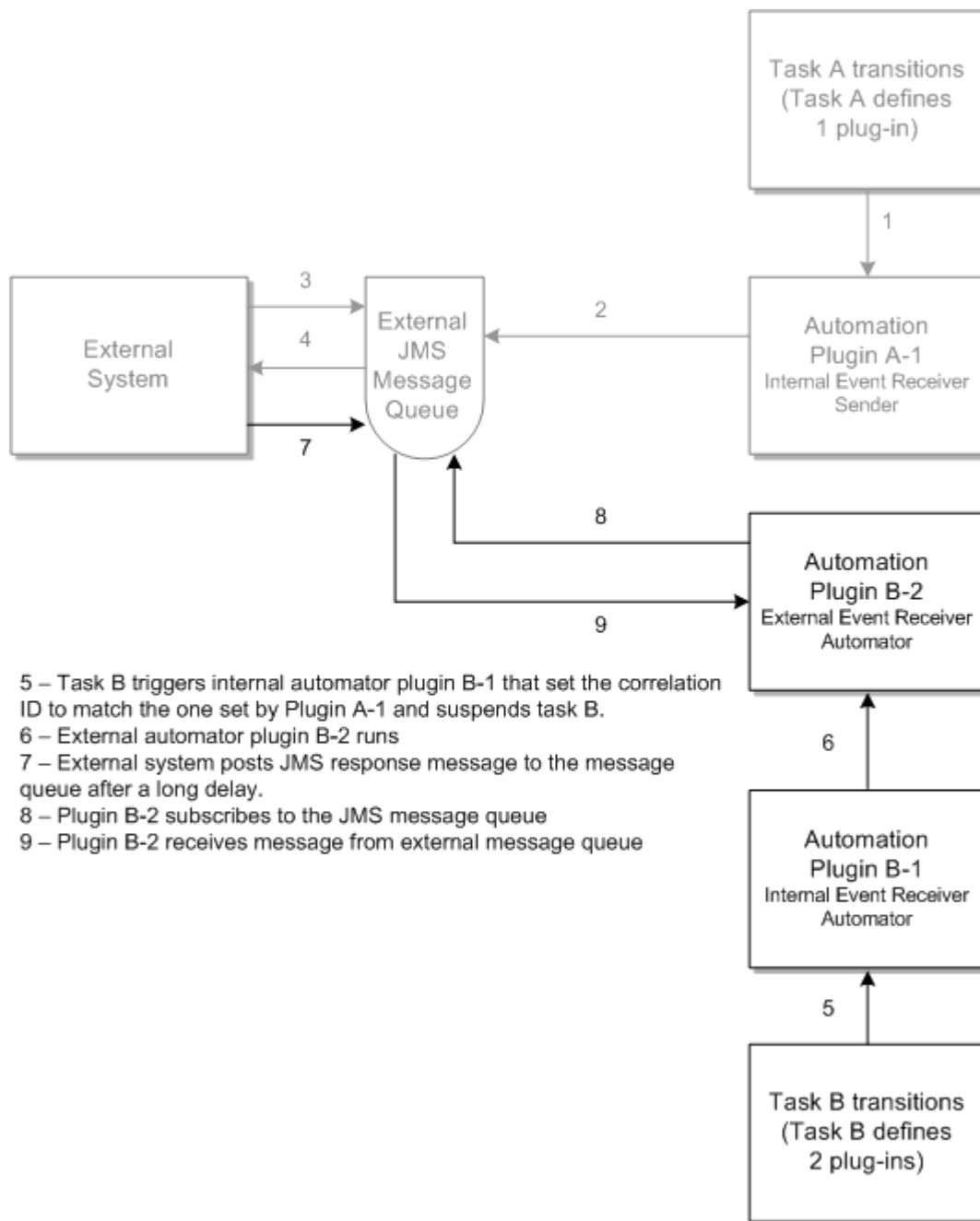
Figure 8–7 Automation Flow: Simple Asynchronous
