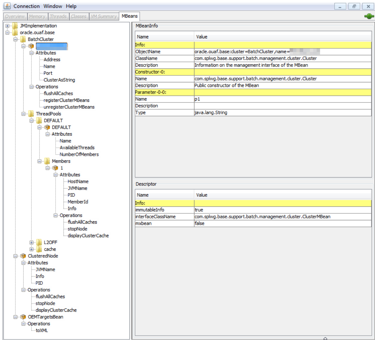
Figure 21 – Example Batch Server Mbeans in jconsole
