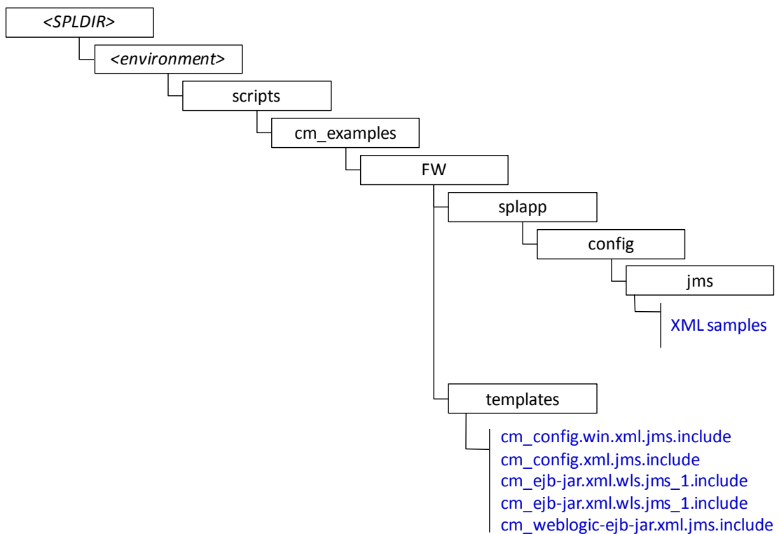
Figure 48 – Custom JMS configuration
