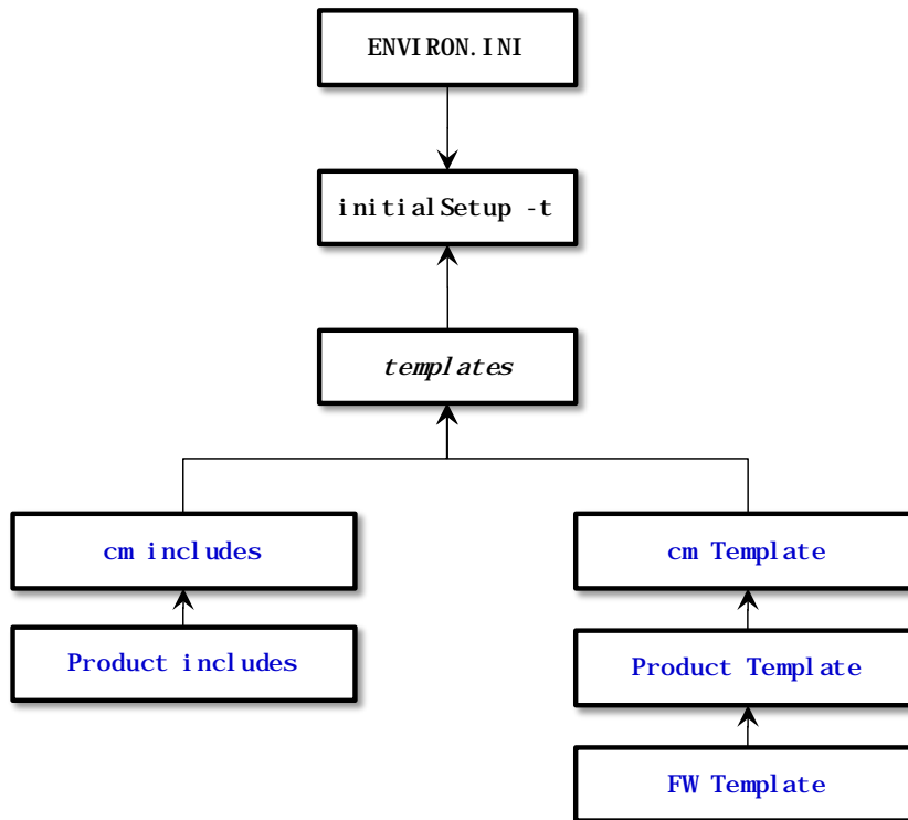
Figure 42 – Template Hierarchy
