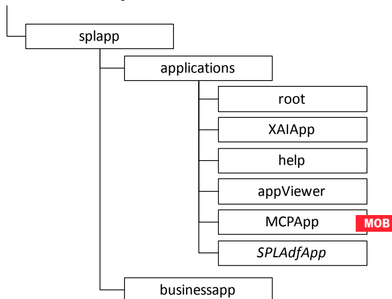
Figure 40 – Expanded Format
