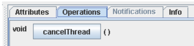
Figure 48 – Example cancelThread
