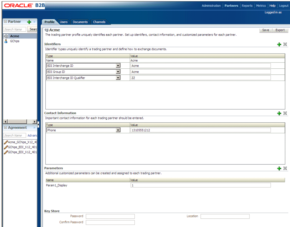
Figure 2-11 Configuring Trading Partners
