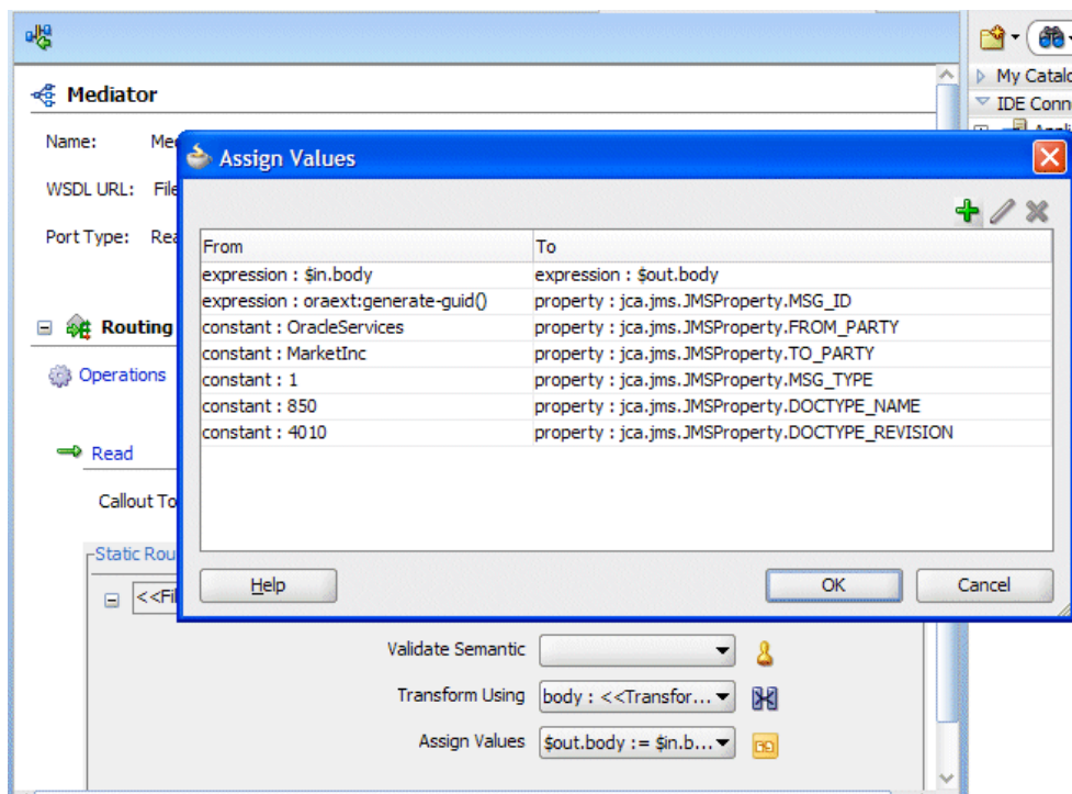
Figure 2-15 Adding JCA JMS Properties in the Assign Values Dialog
