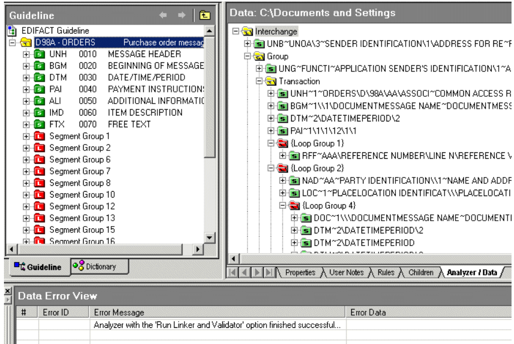
Figure 3-16 Results from the Analyzer
