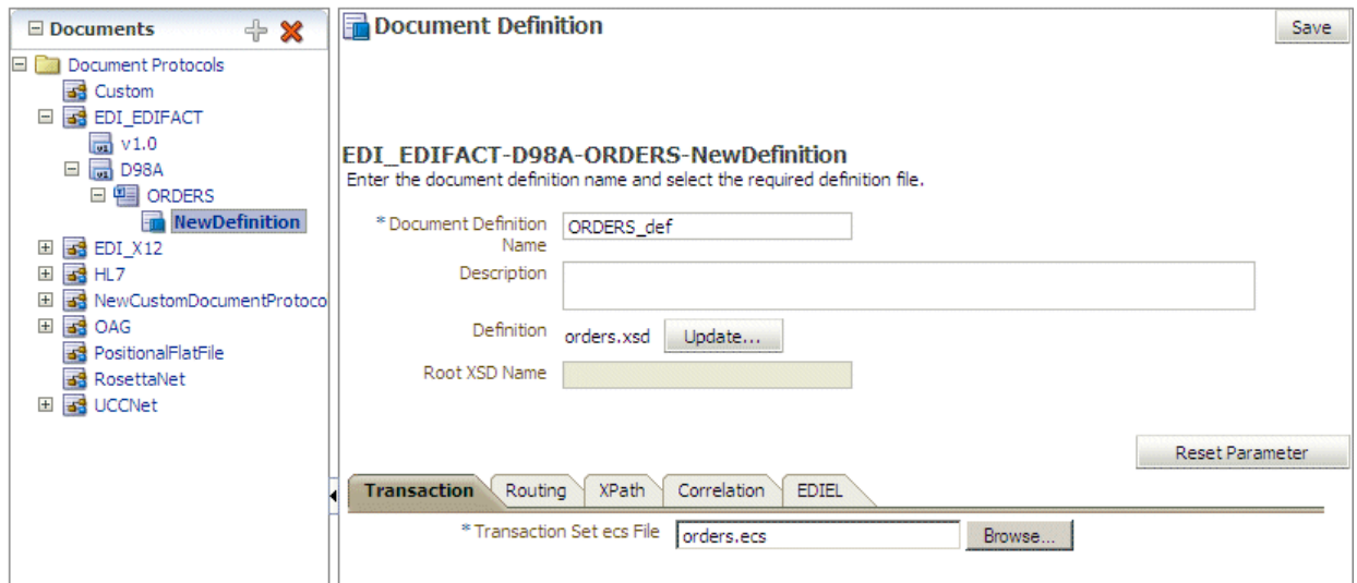
Figure 4-9 Entering Document Definition Parameter Information
