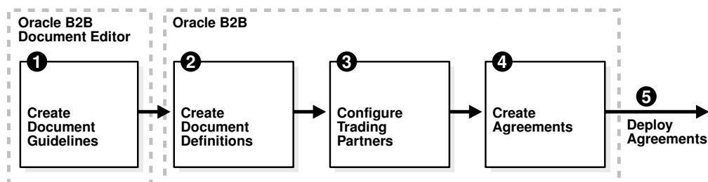
Figure 4-1 Oracle B2B Process Flow
