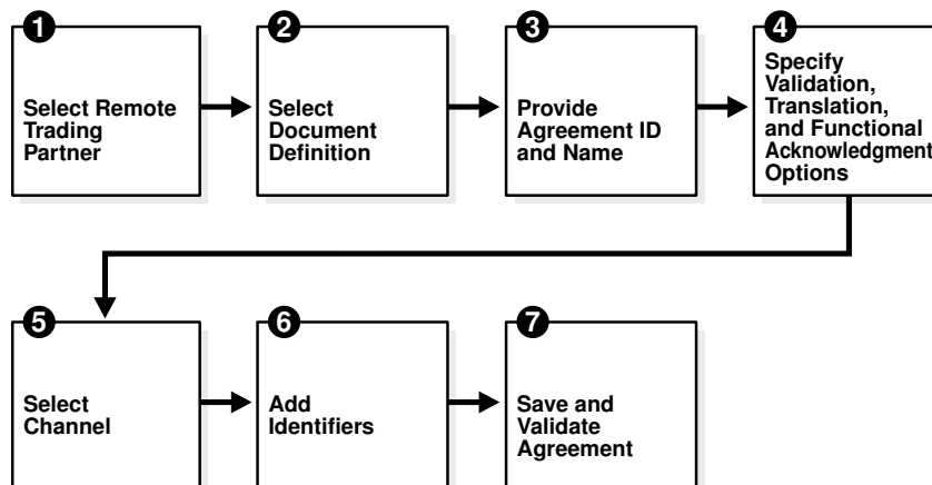
Figure 6-3 Steps to Creating an Agreement (Workflow Overview)
