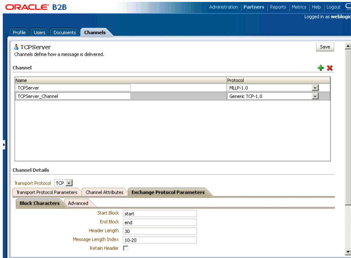
Figure 5-21 Parameters for Generic TCP
