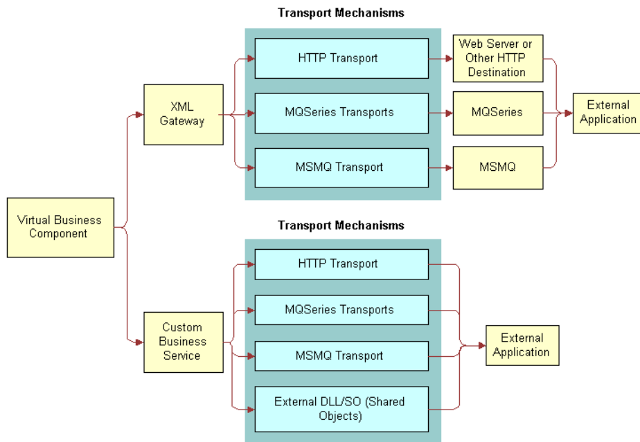
Figure 37. Two Approaches to Building Virtual Business Components
