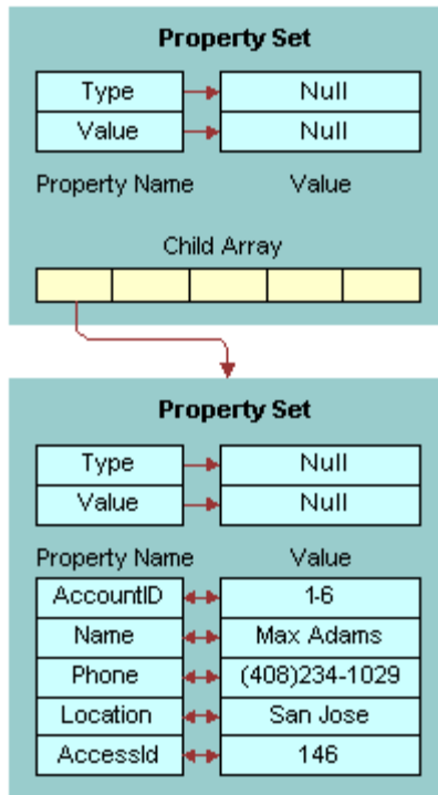
Figure 38. Delete Input Property Set
