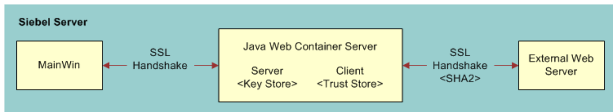
Figure 25. Siebel outbound web service configuration for SHA2
