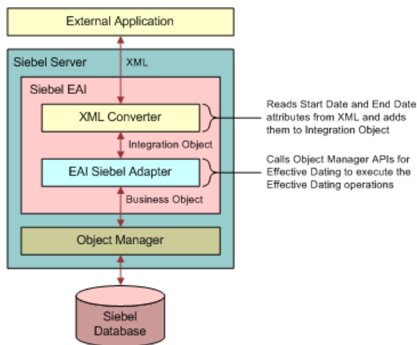
Figure 35. Effective Dating Overview
