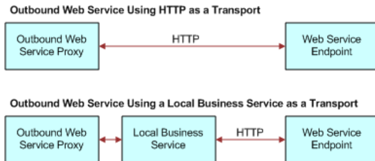
Figure 27. Local Business Service Used as a Transport
