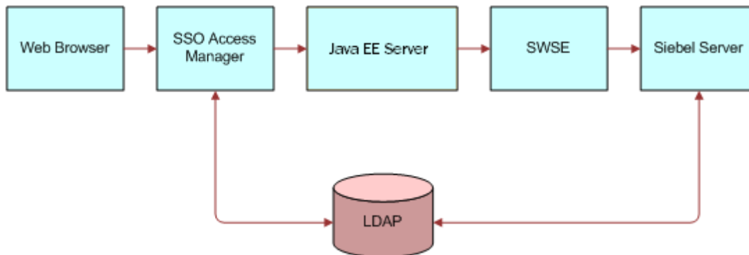
Figure 32. Web Single Sign-On Scenario
