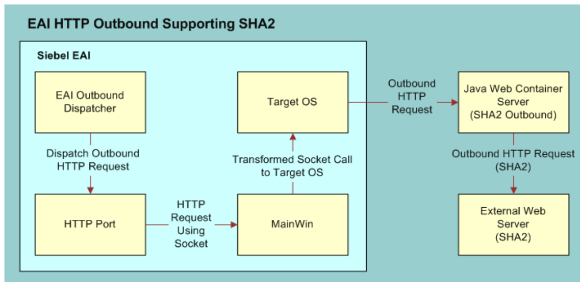
Figure 26. Detailed Siebel outbound web service configuration for SHA2
