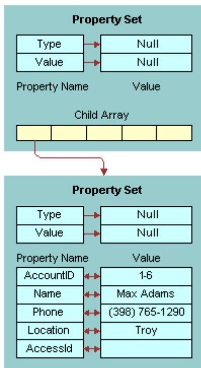
Figure 43. Insert Input Property Set
