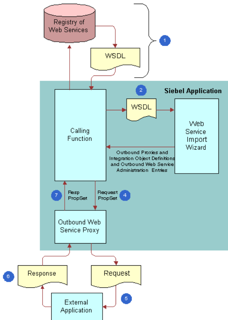
Figure 28. Invoking an External Web Service
