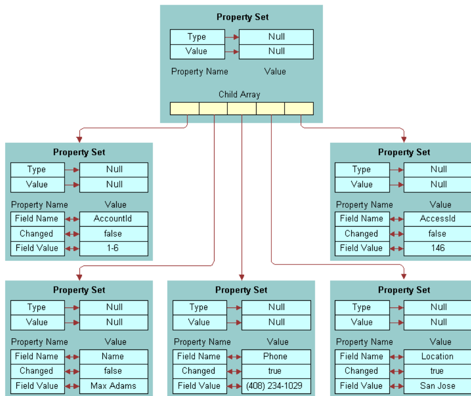
Figure 49. Update Input Property Set
