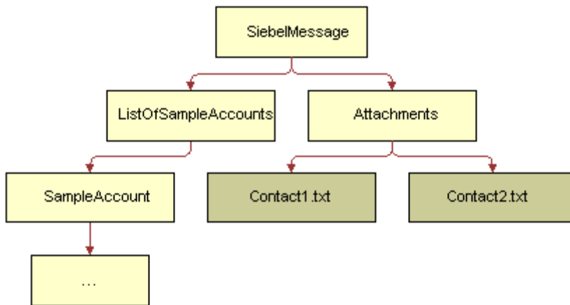
Figure 51. Sample Account with Attachments as Input to the MIME Hierarchy Converter
