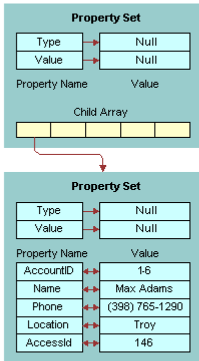
Figure 44. Insert Output Property Set
