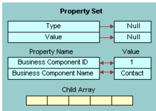
Figure 45. PreInsert Input Property Set
