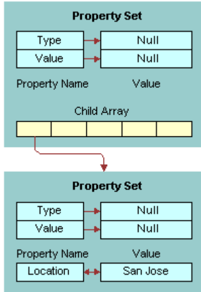
Figure 46. PreInsert Output Property Set
