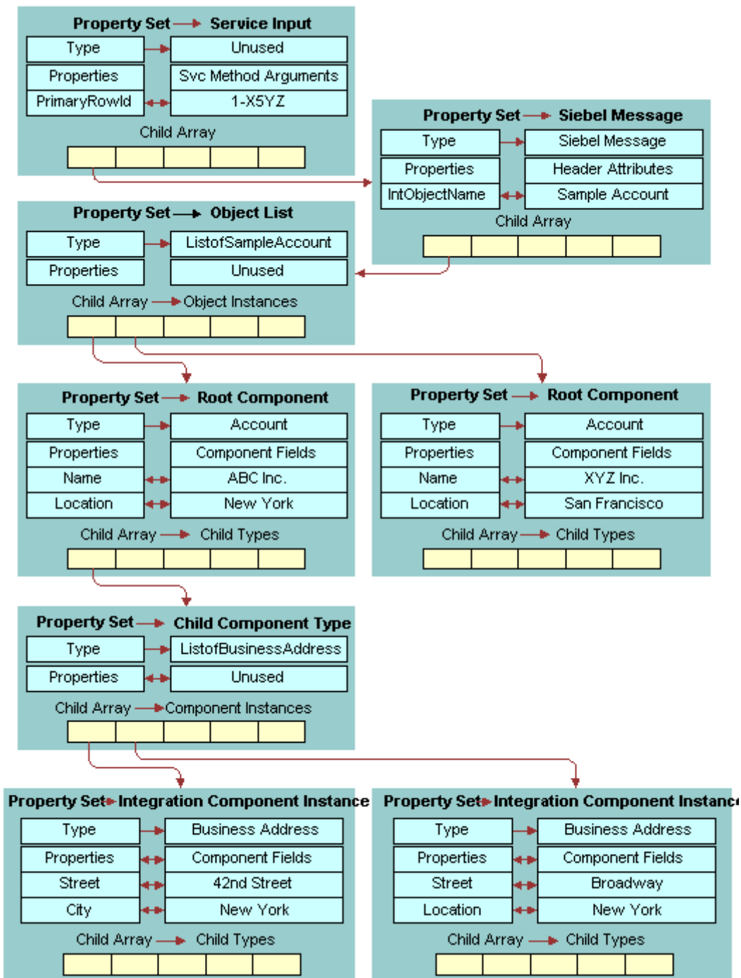
Figure 55. Partial Instance of Sample Account Integration Object
