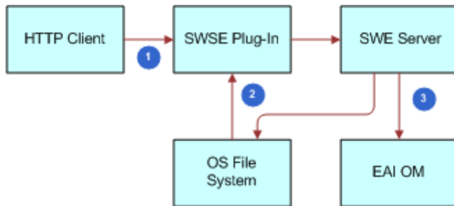
Figure 33. Request-Response Cycle for an Inbound EAI Streaming Request
