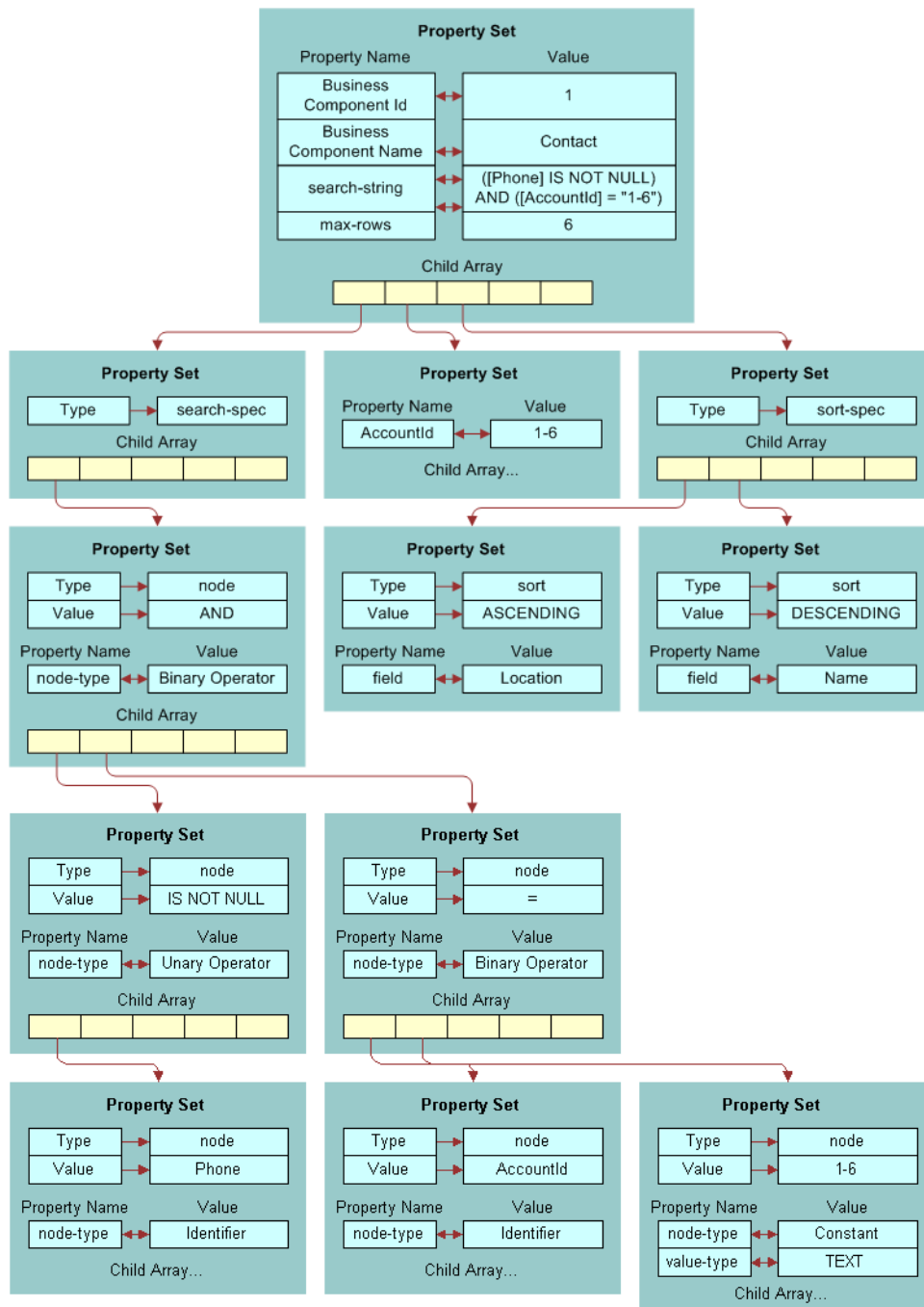
Figure 47. Query Input Property Set
