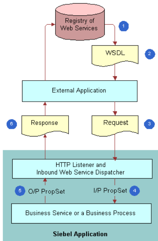
Figure 29. Invoking a Siebel Web Service
