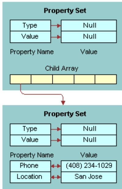
Figure 50. Update Output Property Set
