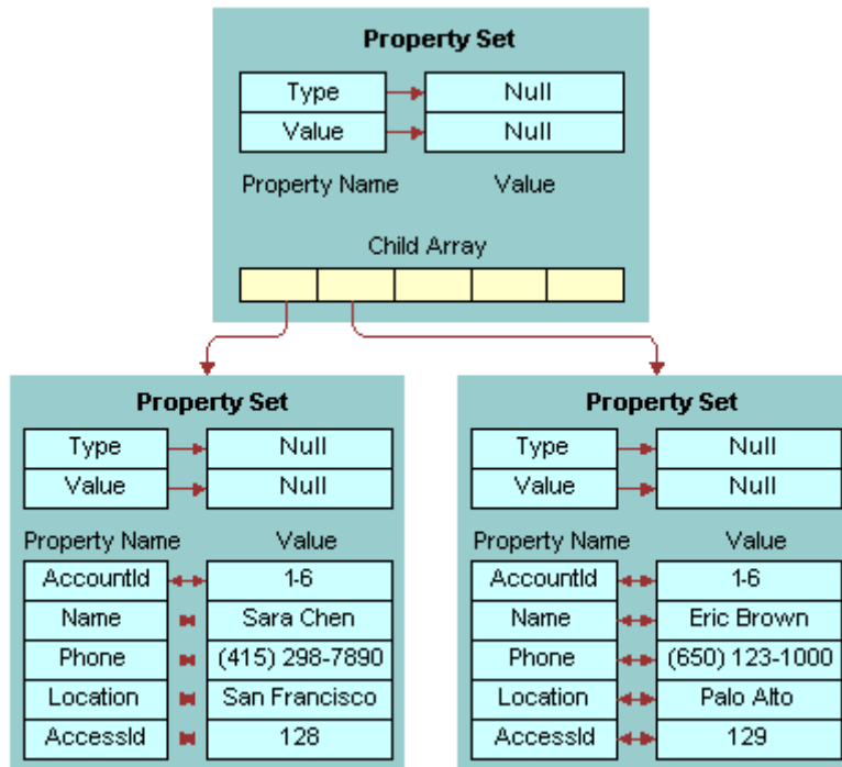
Figure 48. Query Output Property Set
