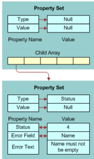
Figure 40. Error Return Property Set
