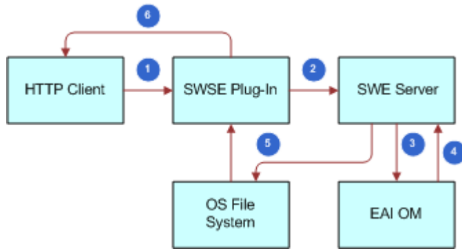
Figure 34. Request-Response Cycle(s) for an Outbound Streaming Response
