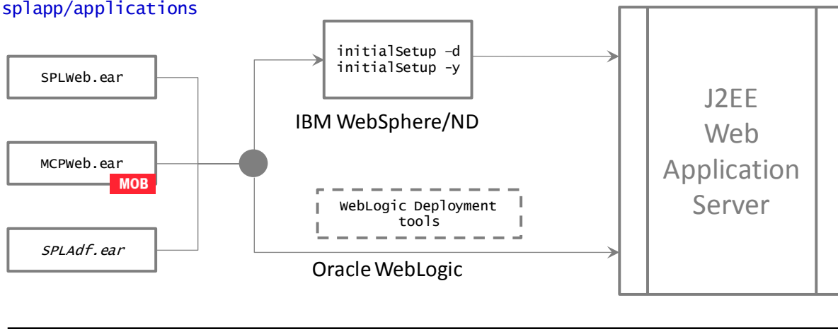
Figure 25 – Web Application Server Deployment Process
