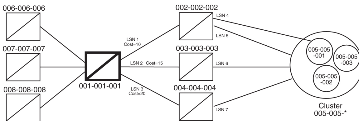
Figure 15: Cluster Management
