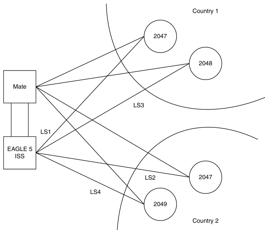
Figure 3: Network Example #1
