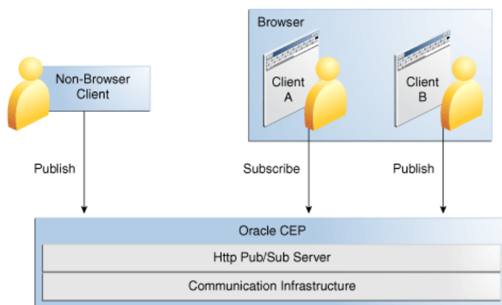
Figure 13-1 HTTP Publish-Subscribe Server in Oracle Stream Analytics
