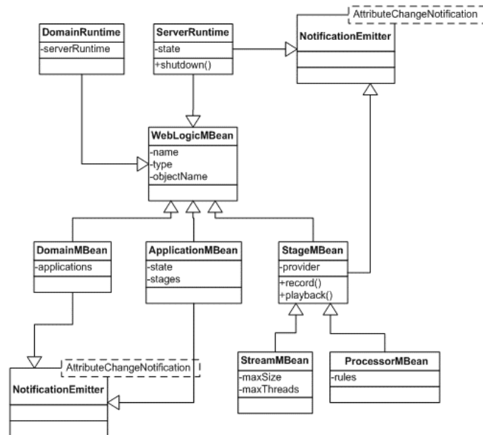
Figure 11-1 Event Processing MBean Object Model
