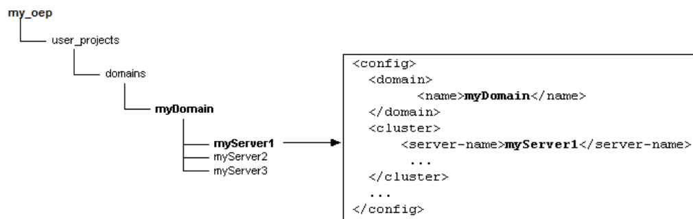
Figure 4-1 Multiserver Domain Directory Structure
