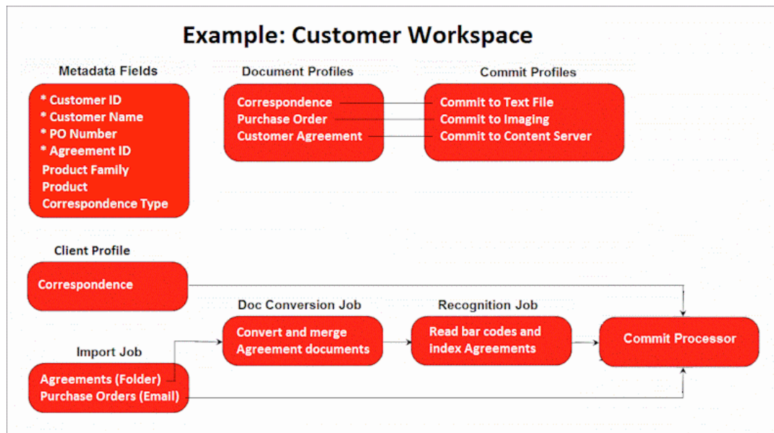
Figure 2-3 Customer Workspace
