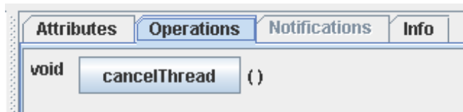
Figure 48 – Example cancelThread
