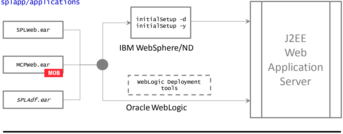
Figure 25 – Web Application Server Deployment Process
