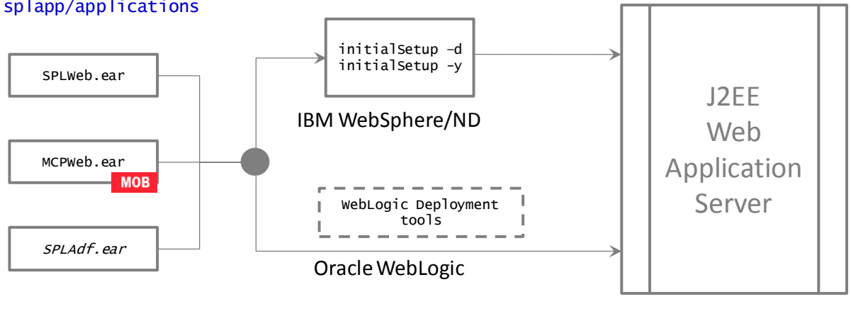
Figure 25 – Web Application Server Deployment Process
