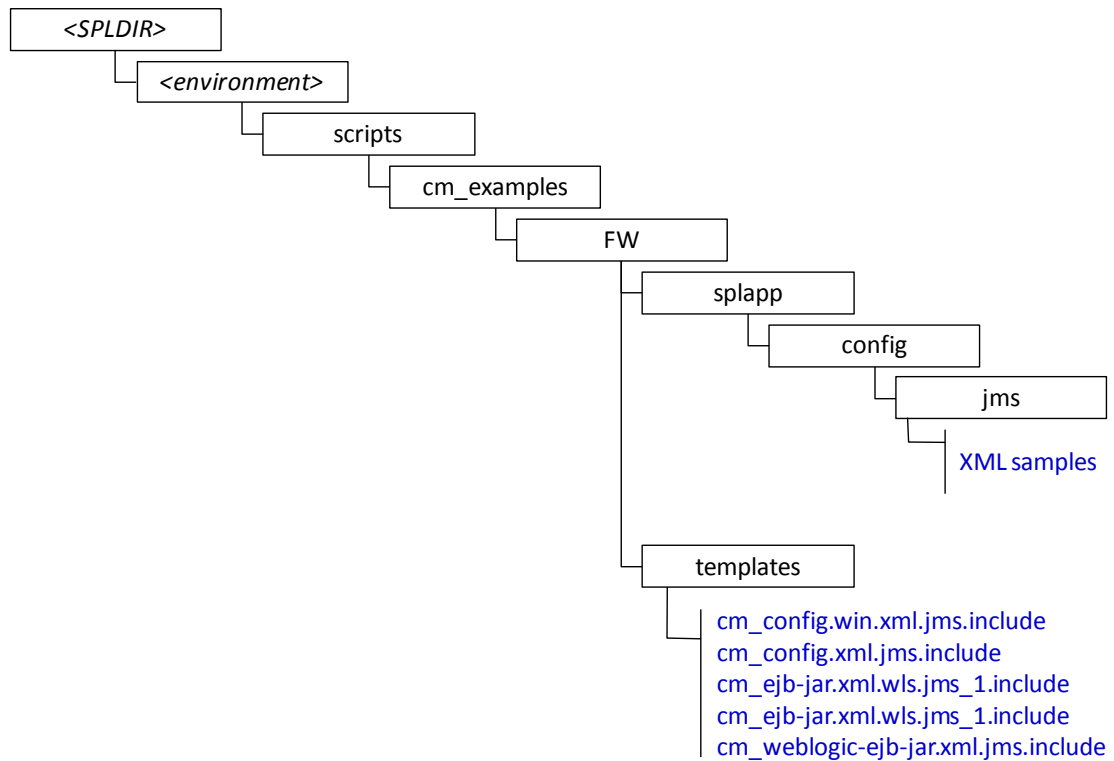
Figure 43 – Custom JMS configuration
