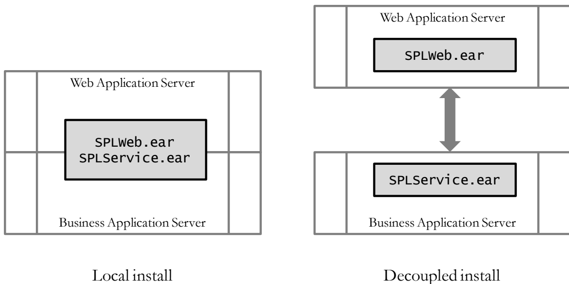
Figure 26 – Installation Modes
