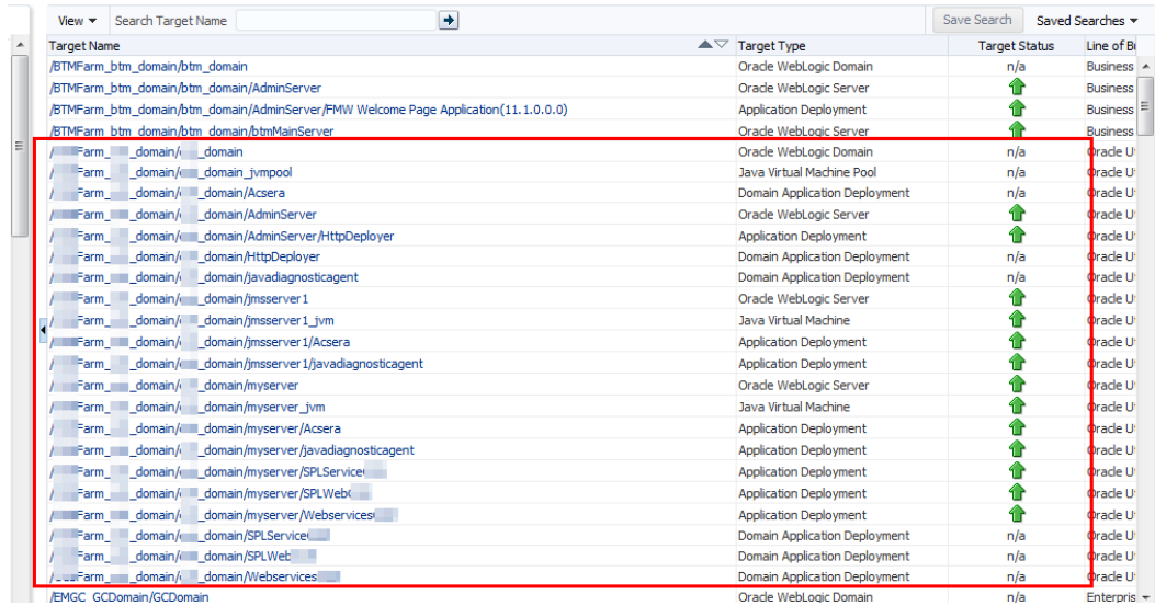
Figure 49 – Oracle WebLogic Targets
