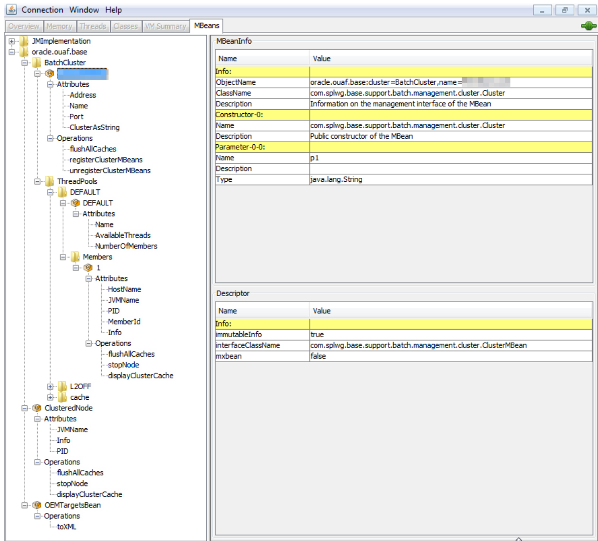
Figure 16 – Example Batch Server Mbeans in jconsole
