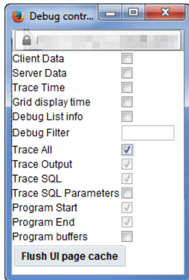
Figure 11 – Debug controls
