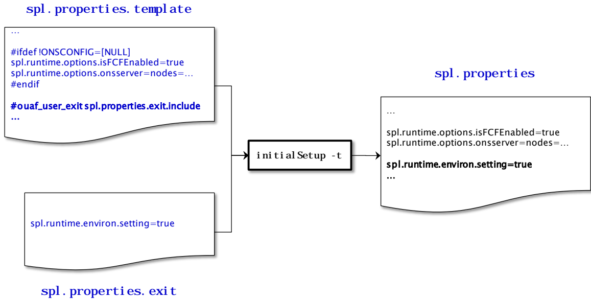
Figure 41 – Include files
