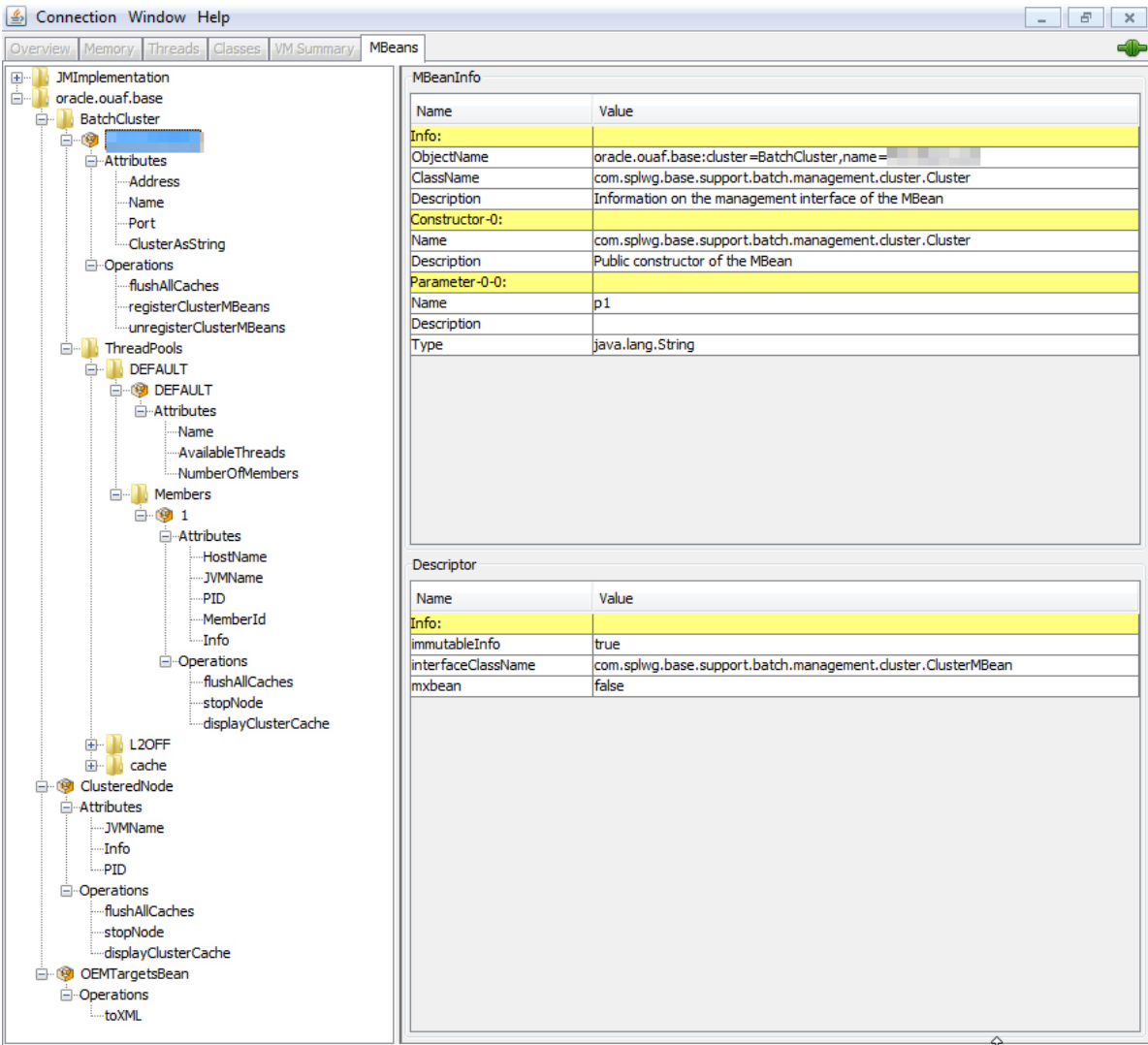
Figure 16 – Example Batch Server Mbeans in jconsole
