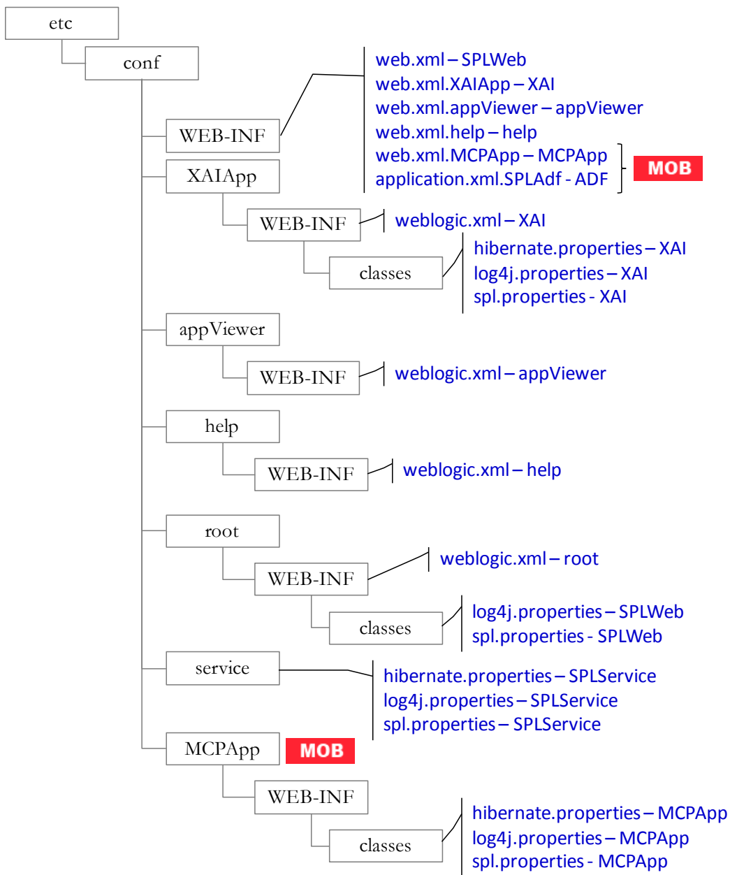
Figure 23 – Configuration File hierarchy
