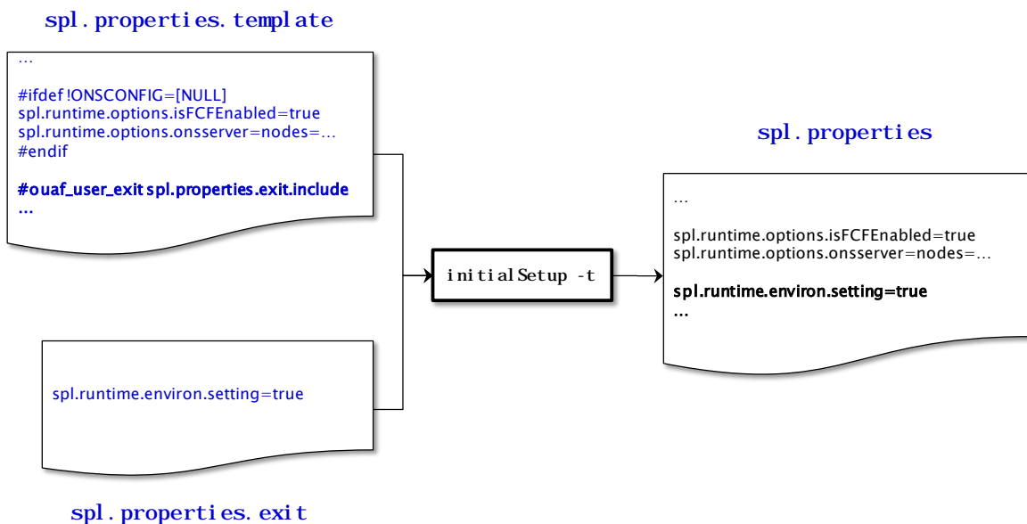
Figure 41 – Include files
