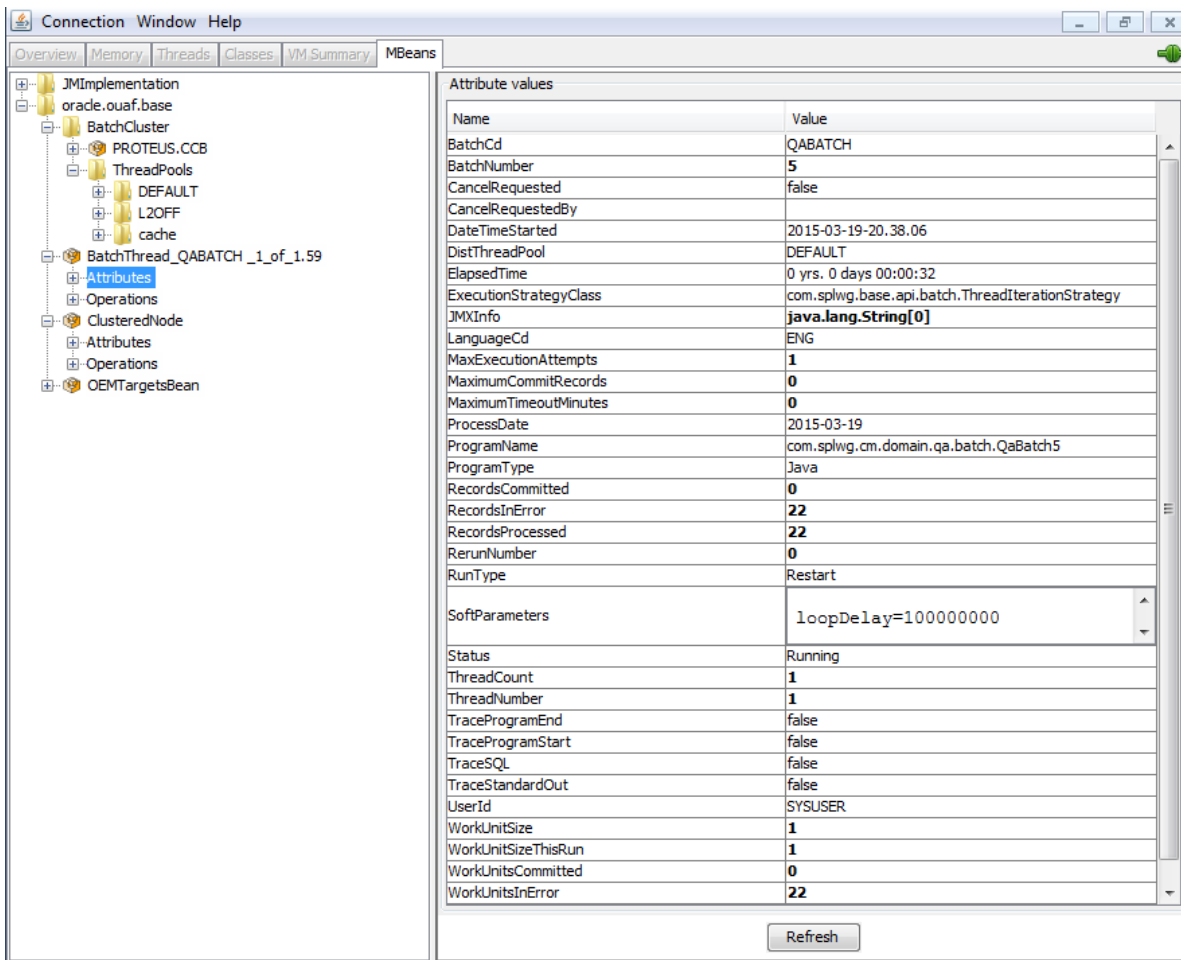
Figure 17 – Example Batch Thread Mbean in jconsole
