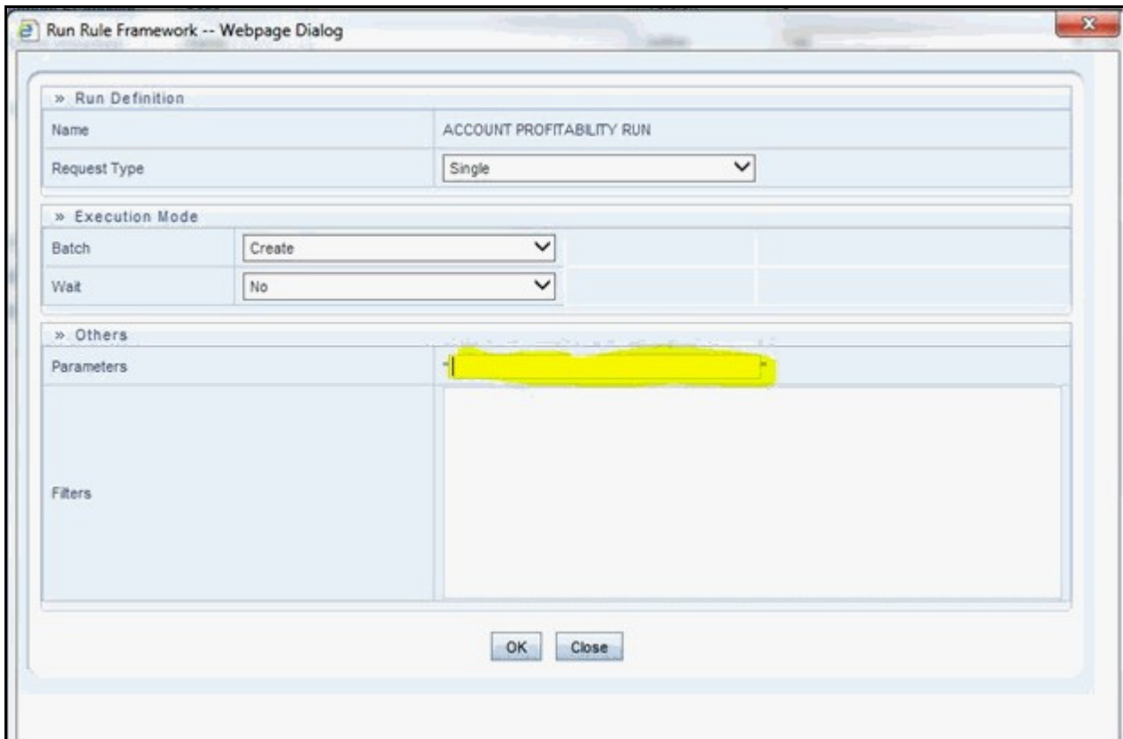
Figure 72. Run Parameters
