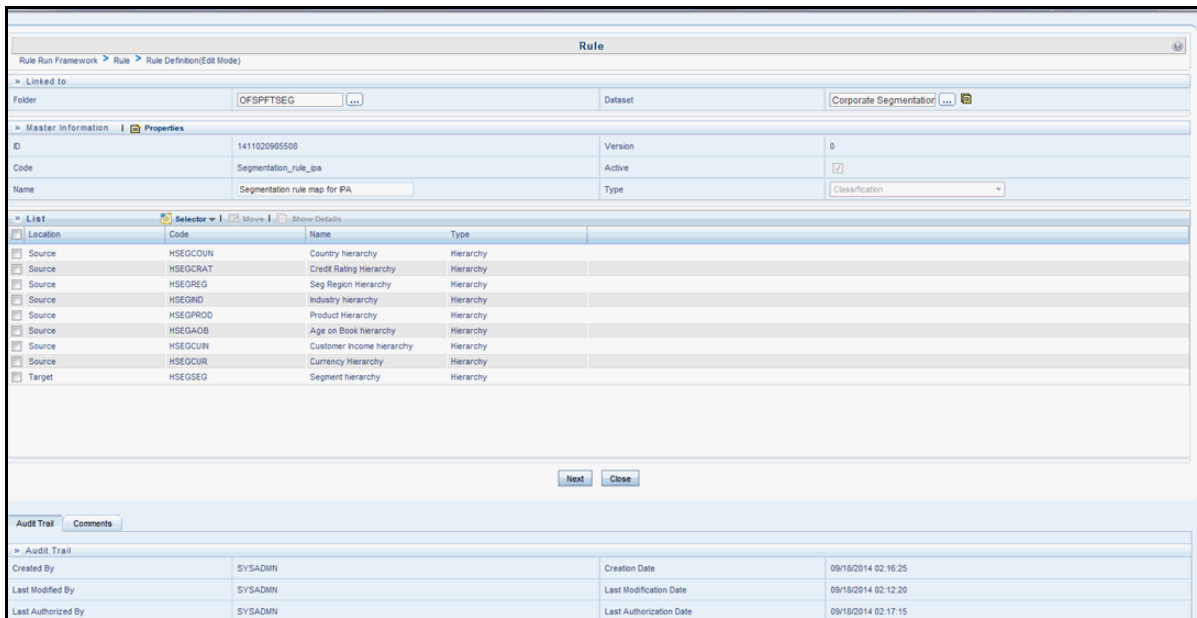
Figure 61. Edit Rule
