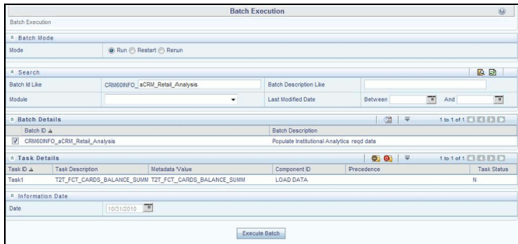
Figure 33. aCRM_Retail_Analysis - Task1
