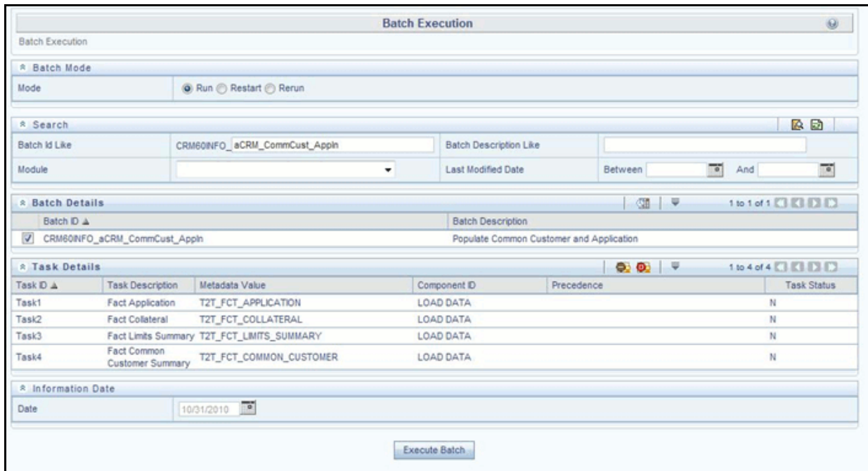
Figure 36. aCRM_CommCust_Appln - Task1
