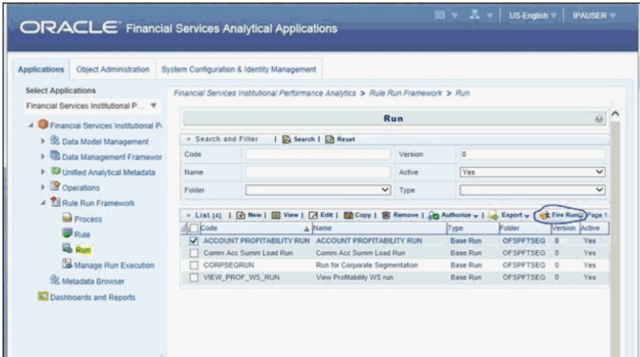
Figure 71. Fire Run
