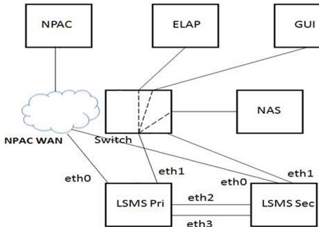
Figure 2-3 Physical Port Assignments - E5-APP-B Segmented Configuration
