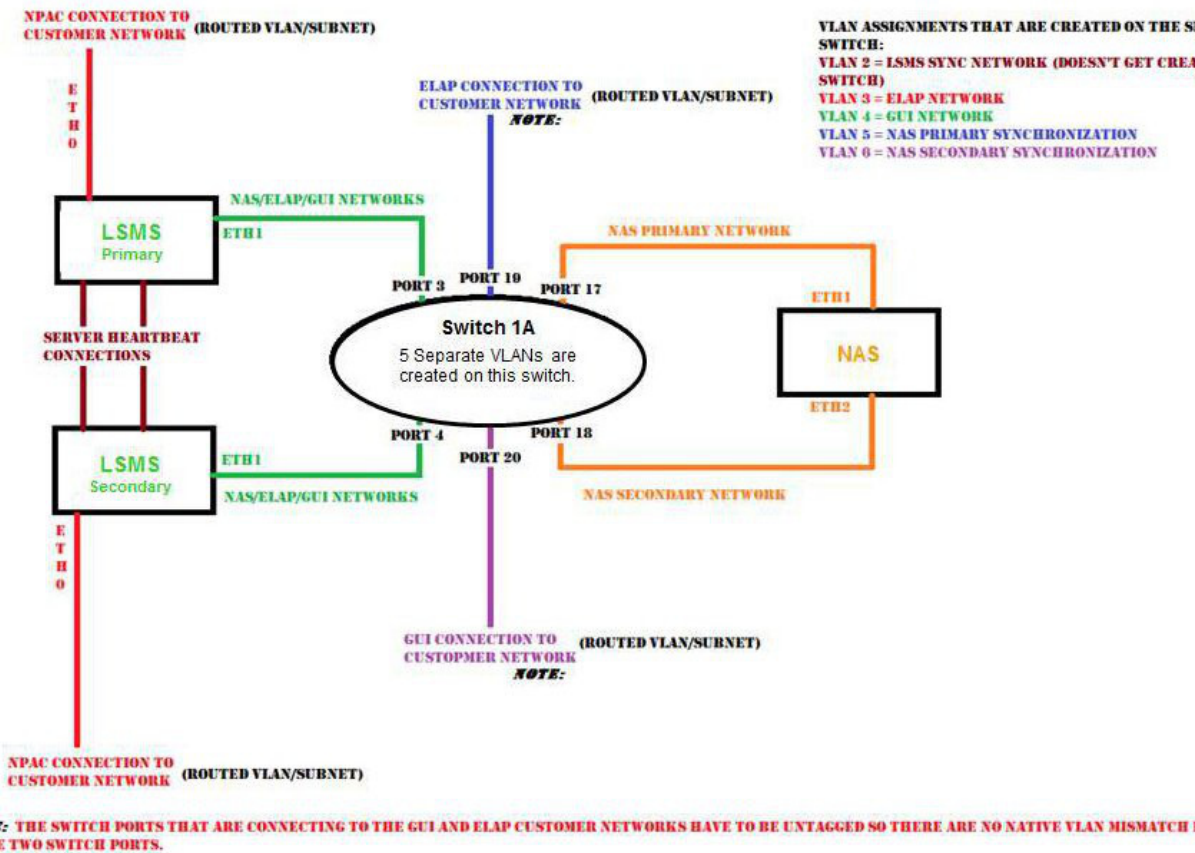
Figure 2-4 LSMS Configuration: Segmented Configuration
