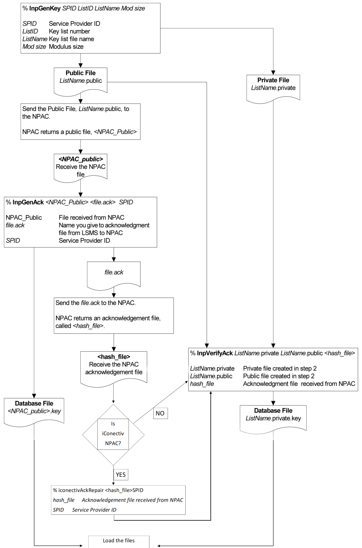
Figure 3-30 Flowchart for Generating a Key List
