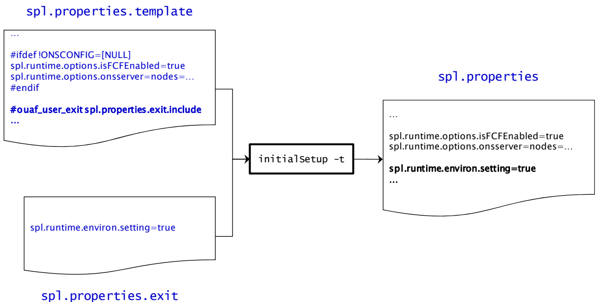
Figure 40 – Include files
