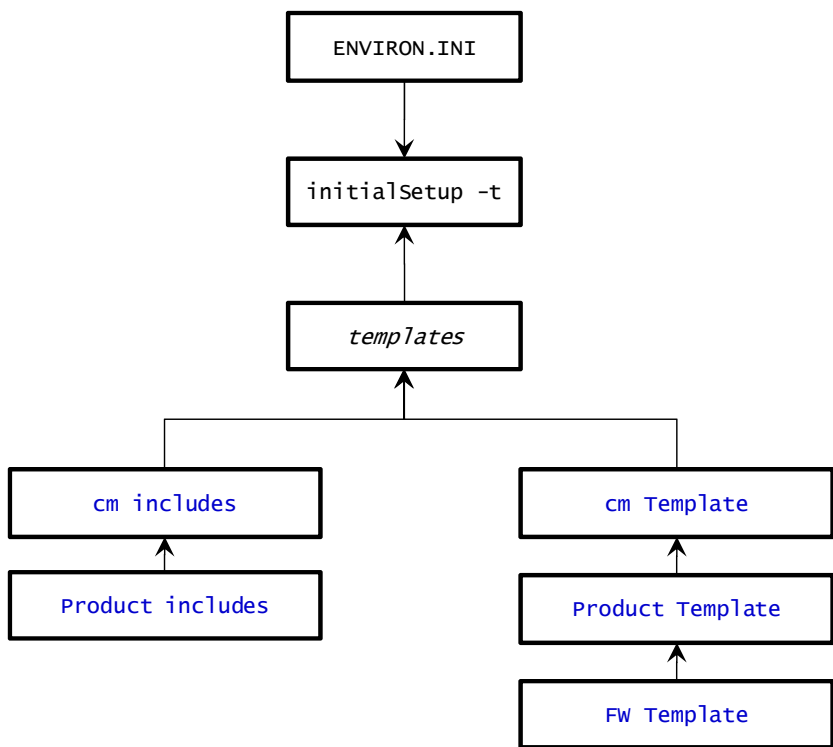
Figure 41 – Template Hierarchy
