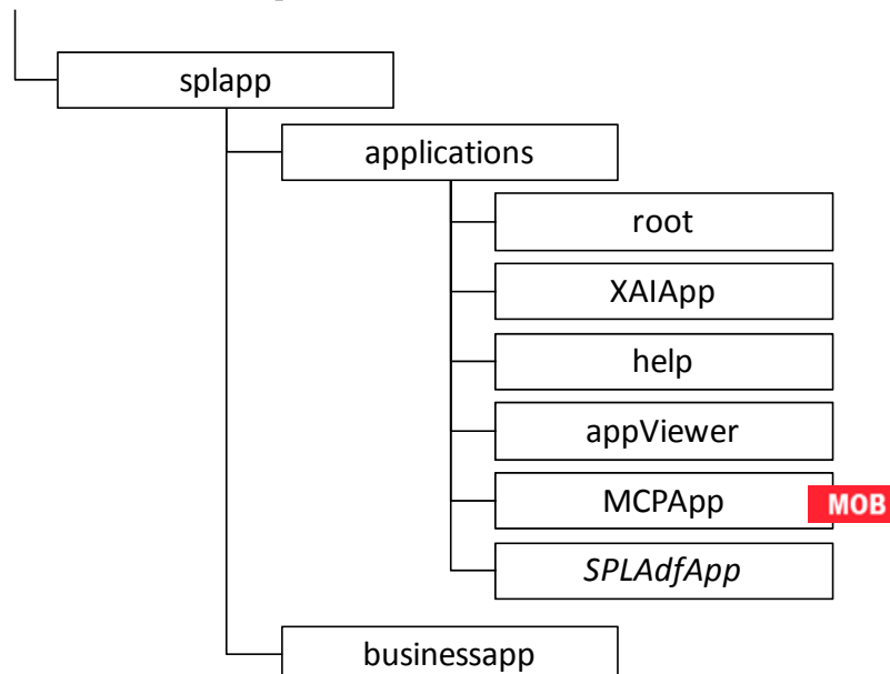
Figure 39 – Expanded Format
