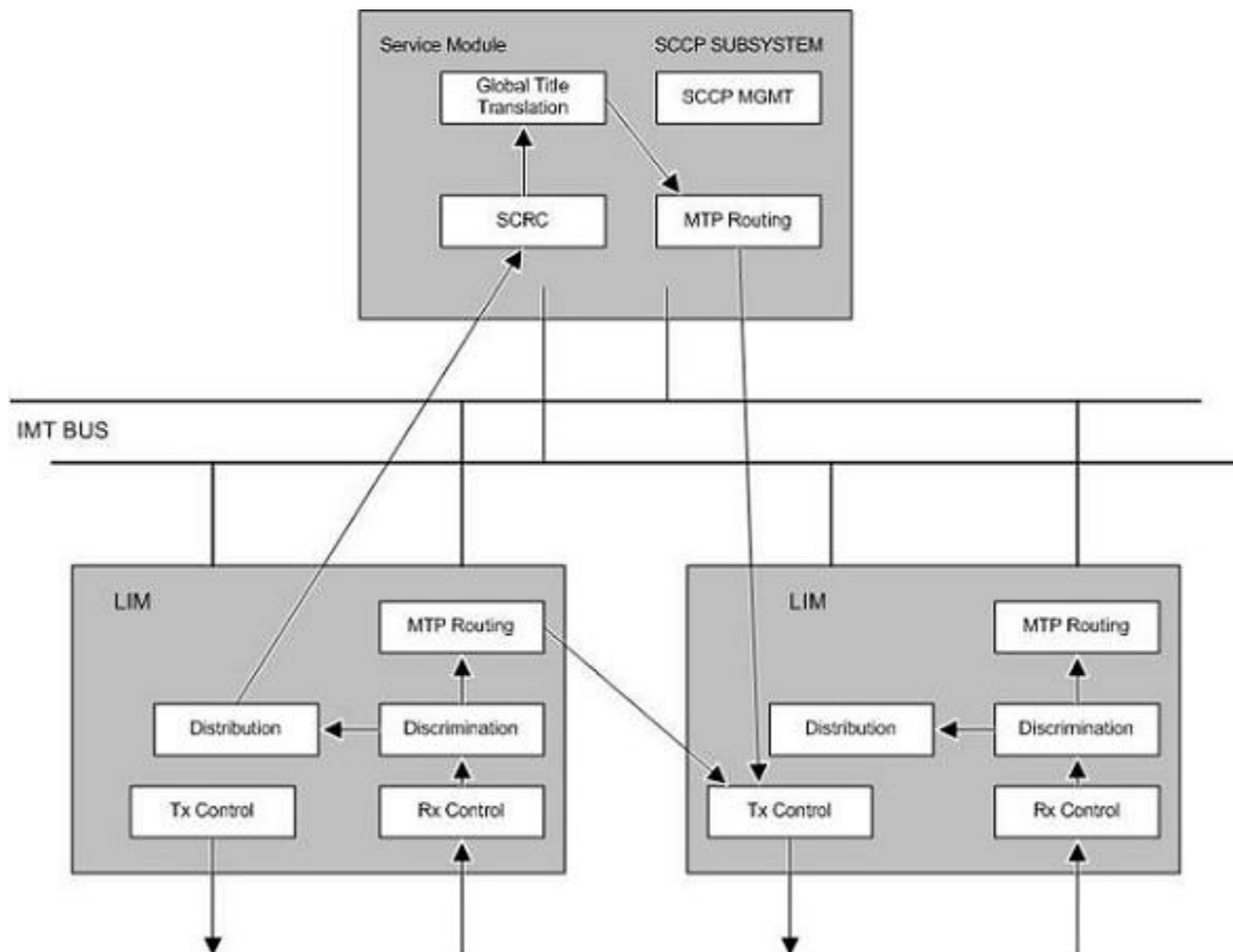
Figure 2-31 SCCP Message Flow through the EAGLE
