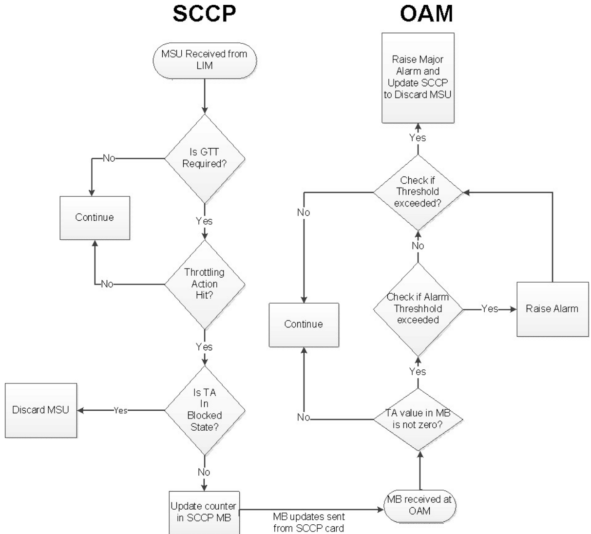
Figure 2-18 Throttling Framework
