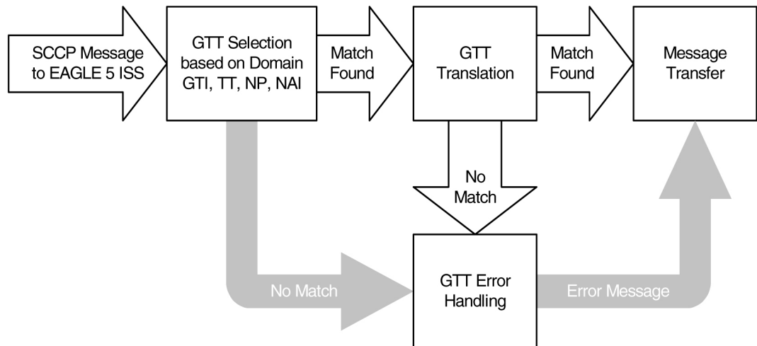
Figure 2-34 EGTT Process
