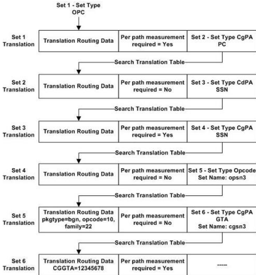
Figure 2-29 GTT Translation Lookup - Exact GTT Action Path Match (with Unspecified GTT Set-Value Combinations)
