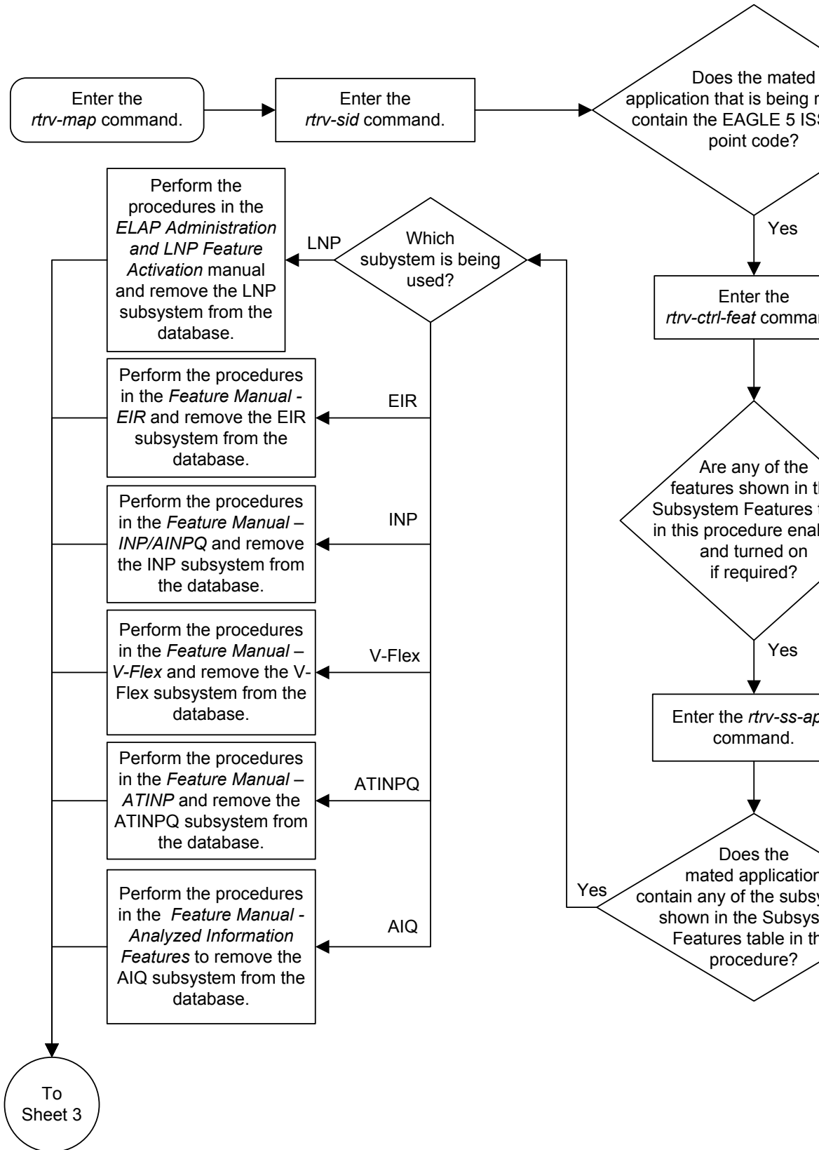
Figure 2-47 Removing a Mated Application
