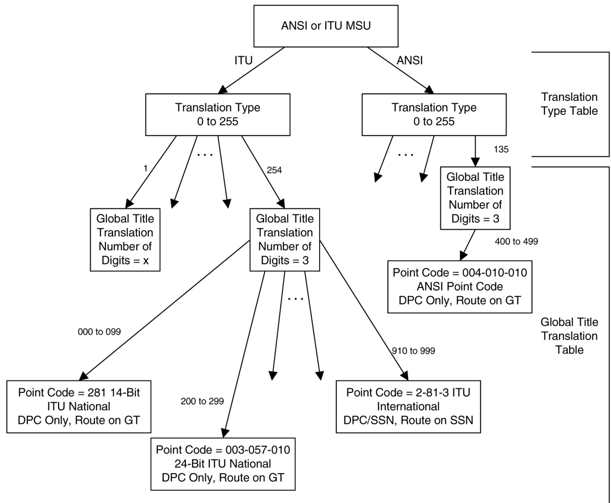
Figure 2-32 Example of Using Translation Type and Global Title Translation Tables
