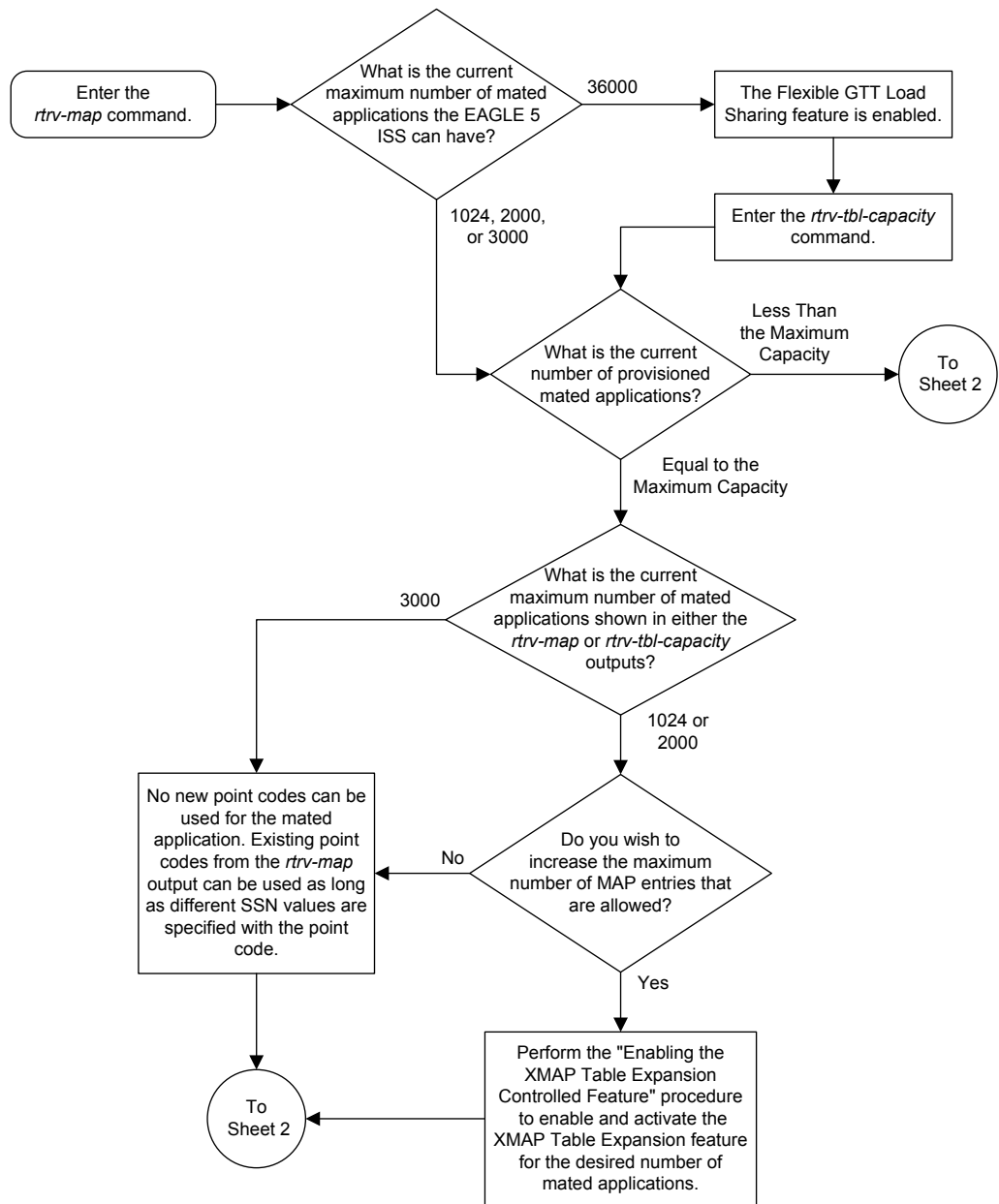
Figure 2-43 Provisioning a Solitary Mated Application
