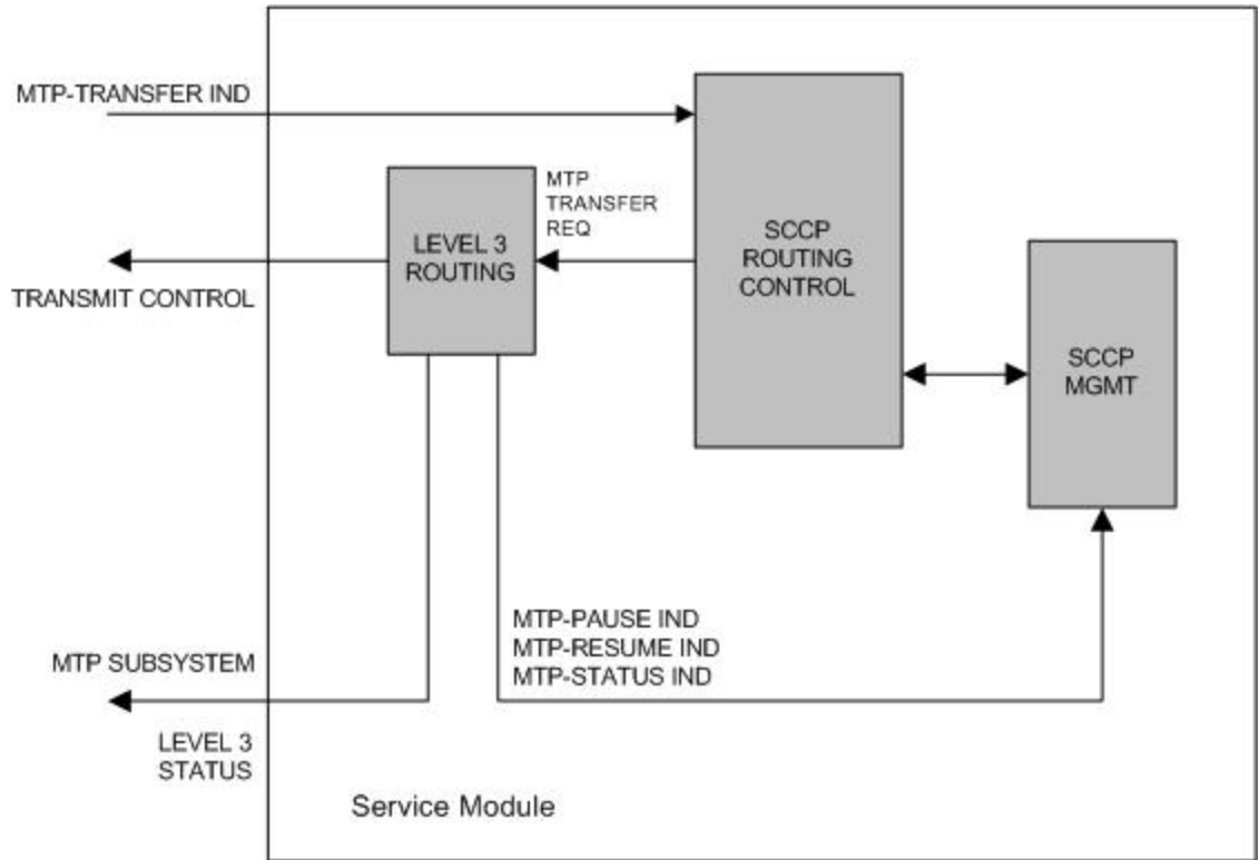
Figure 2-30 Logical View of SCCP Subsystems
