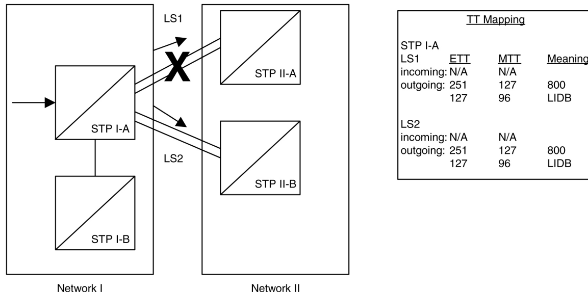
Figure 2-35 An Example of Double Translation Type Mapping
