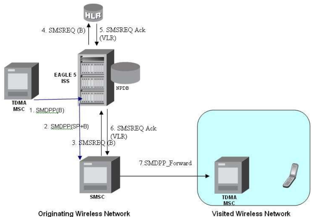
Figure 2-3 MO-Based IS41 SMS NP Call Flow for In-Network Subscriber
