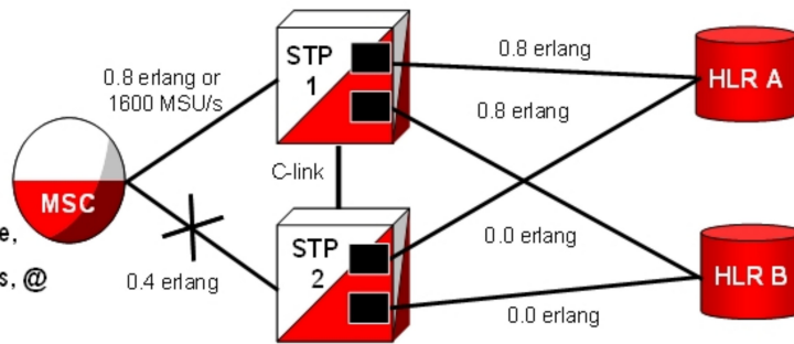
Figure 5-4 EAGLE: Failover at 0.8 Erlang and 1600 MSU/s
