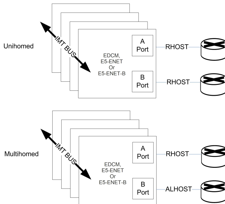
Figure 5-5 Unihoming versus multihoming
