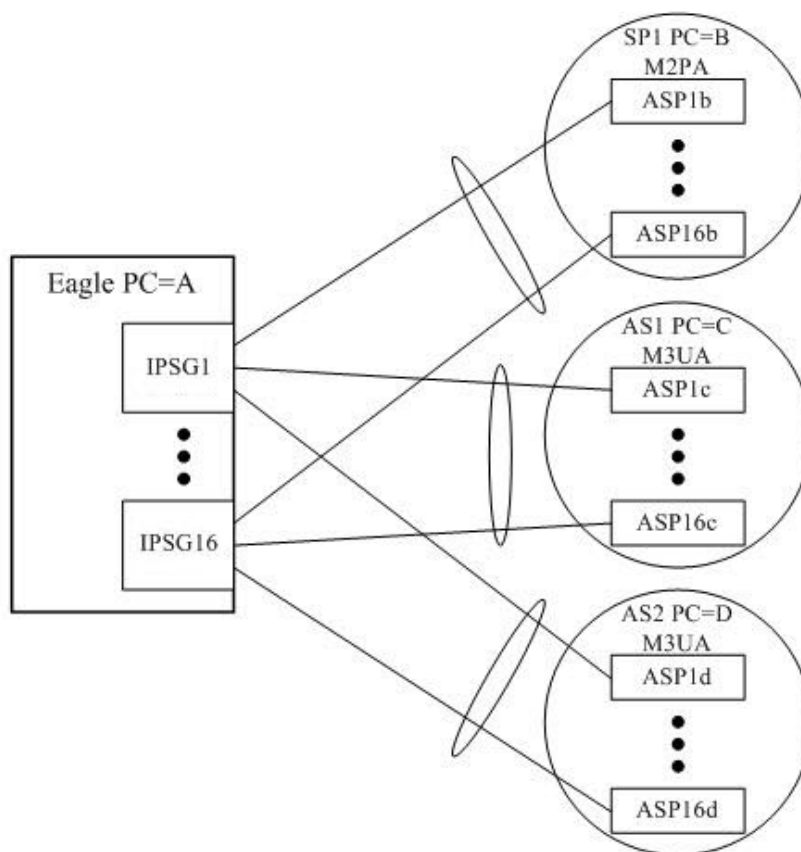
Figure A-1 Example Deployment of IPSG Application
