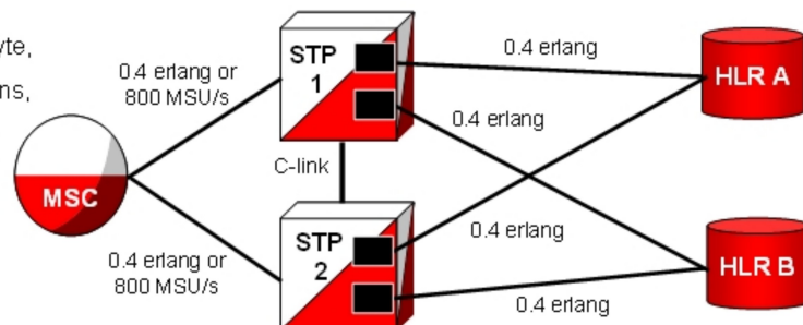
Figure 5-3 SIGTRAN: Every Link at 0.4 Erlang and 800 MSU/s
