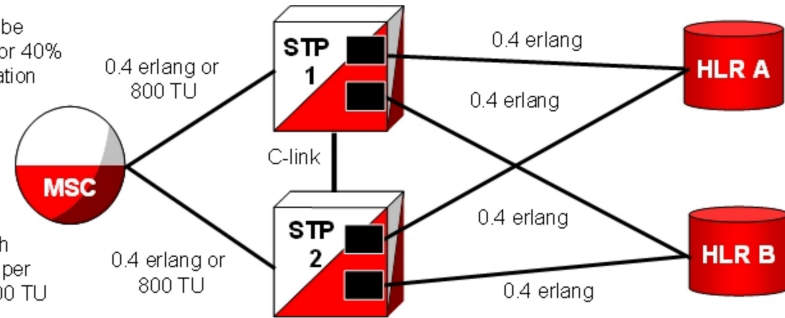
Figure 5-1 SIGTRAN: Every IP Link at 0.4 Erlang
