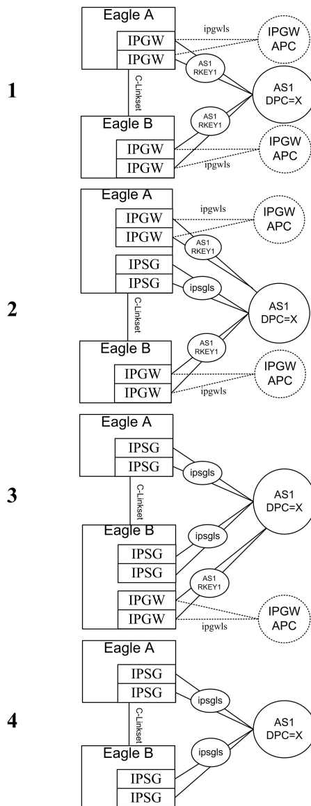
Figure 6-3 IPGWx to IPSP-M3UA Conversion Strategy Example 2A
