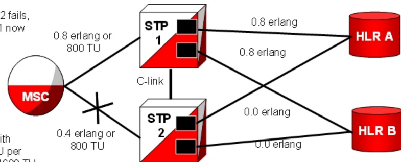
Figure 5-2 SIGTRAN: Failover at 0.8 Erlang
