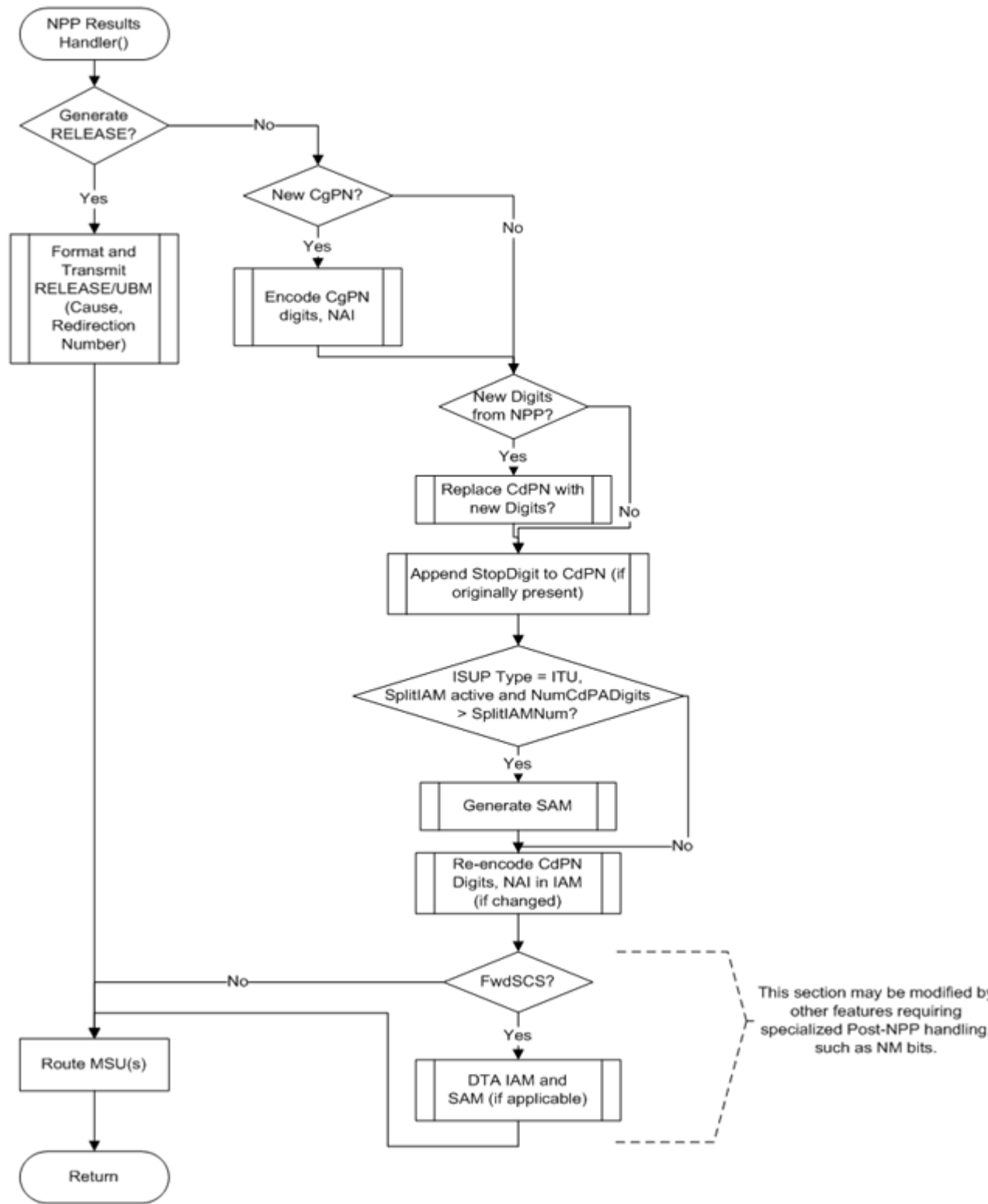
Figure 2-6 TIF Post-NPP Results Handler
