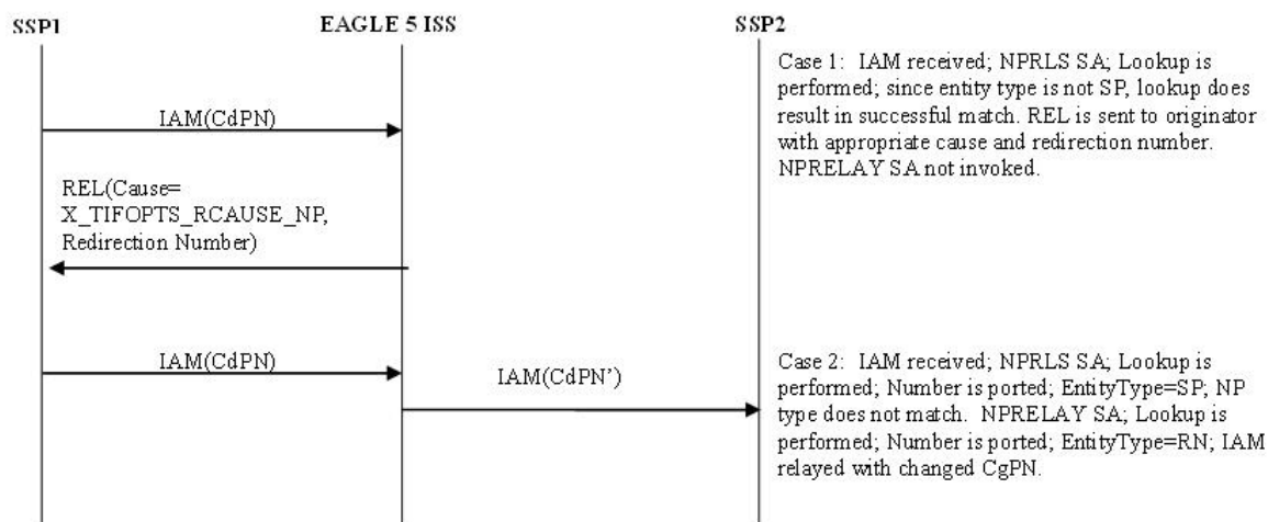
Figure 3-9 ISUP Message Flows for NPRLS + NPRELAY
