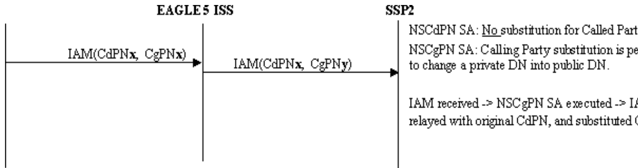
Figure 3-13 ISUP RELAY with TIF NS - No CdPN Substitution
