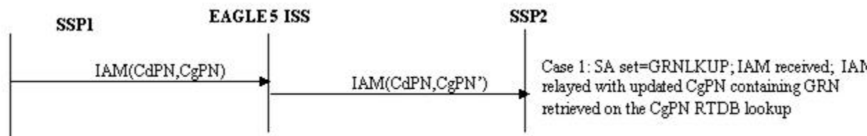
Figure 3-24 ISUP IAM Message Flows for TIF GRN for TIF CgPN Service
