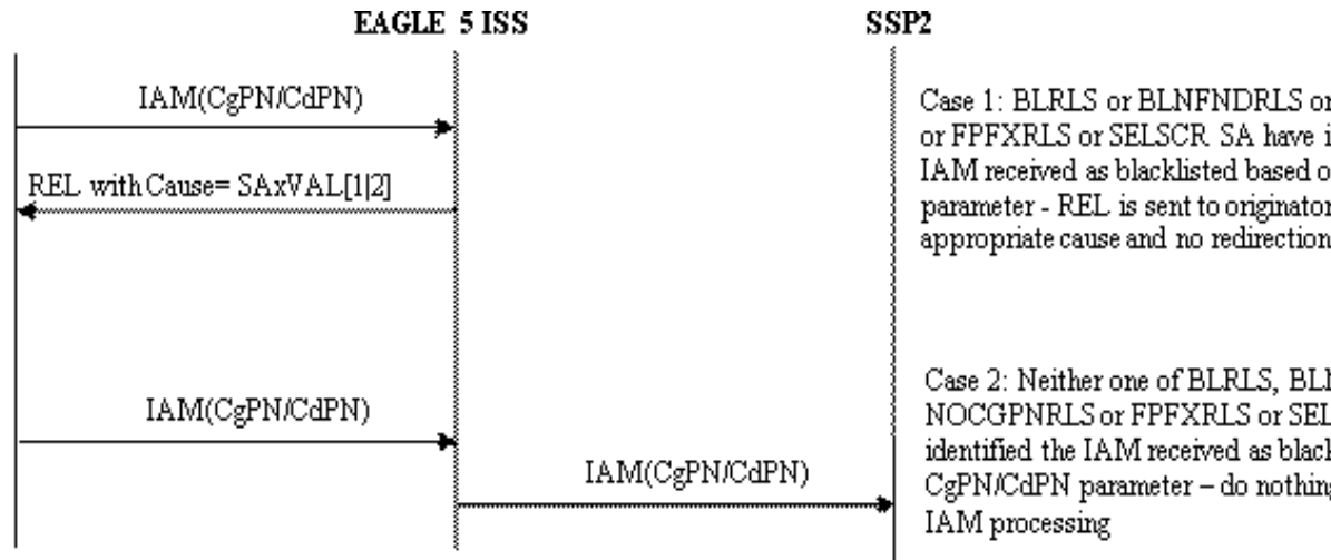
Figure 3-25 TIF Blacklist Basic Message Flow
