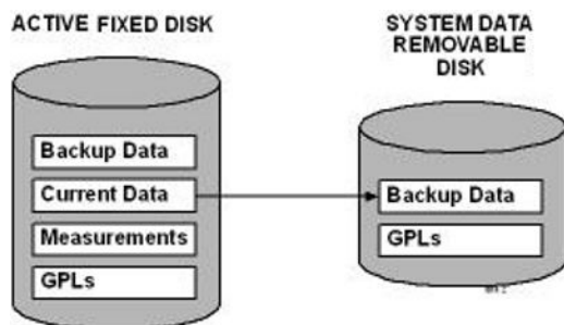
Figure 4-3 chg-db:action=backup:dest=remove
