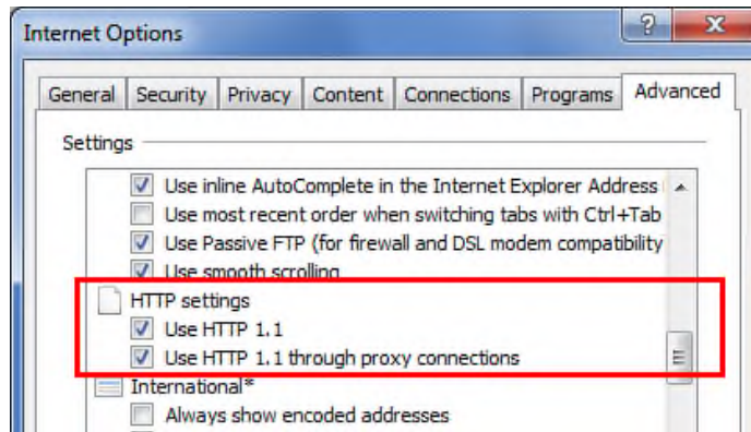
Figure 19 – HTTP 1.1 Settings
