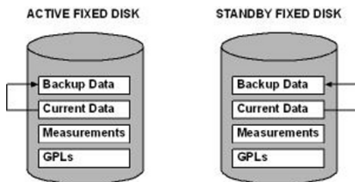
Figure 4-1 chg-db:action=backup:dest=fixed
