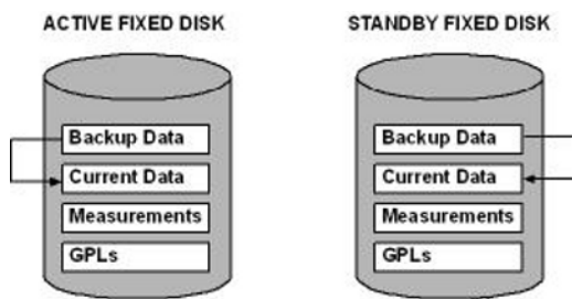
Figure 4-2 chg-db:action=restore:src=fixed
