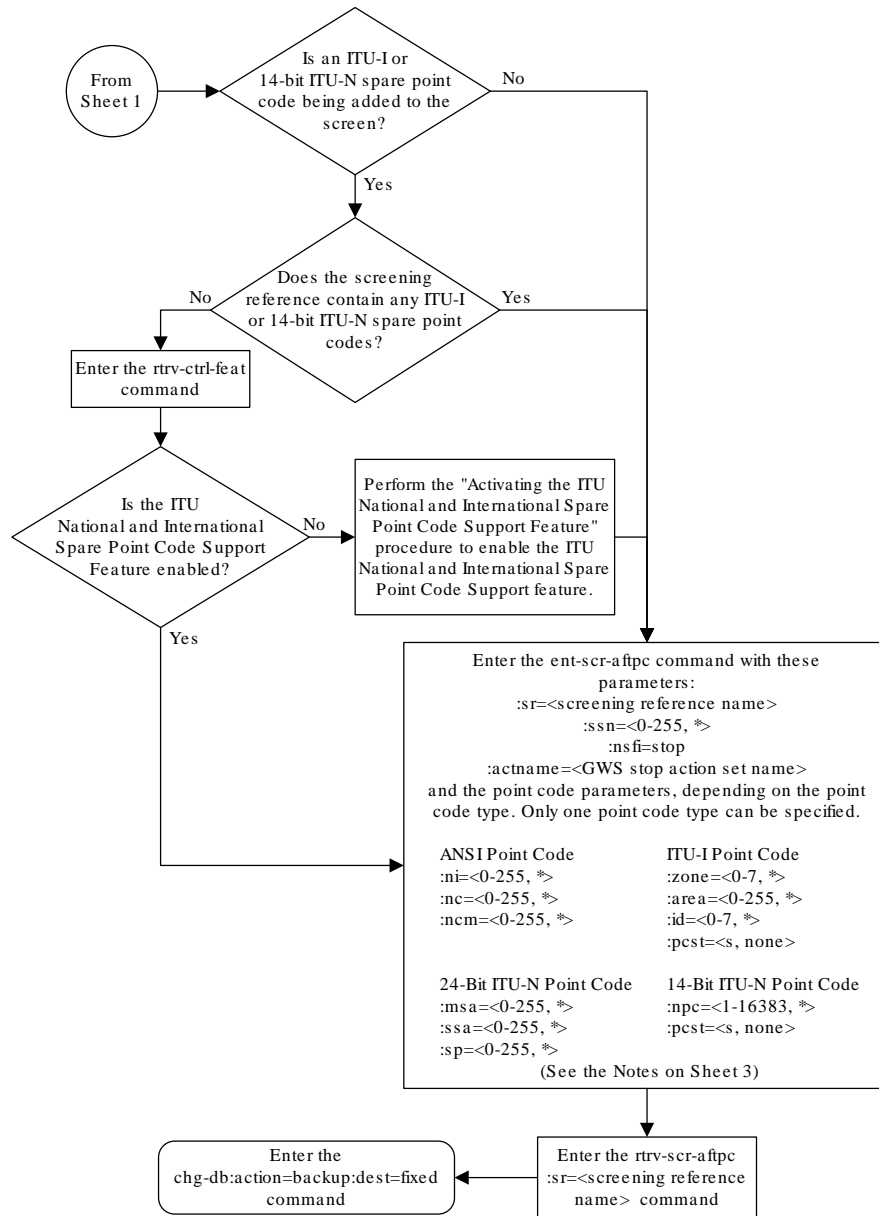
Figure 3-5 Add an Allowed Affected Point Code Screen - Sheet 2 of 3
