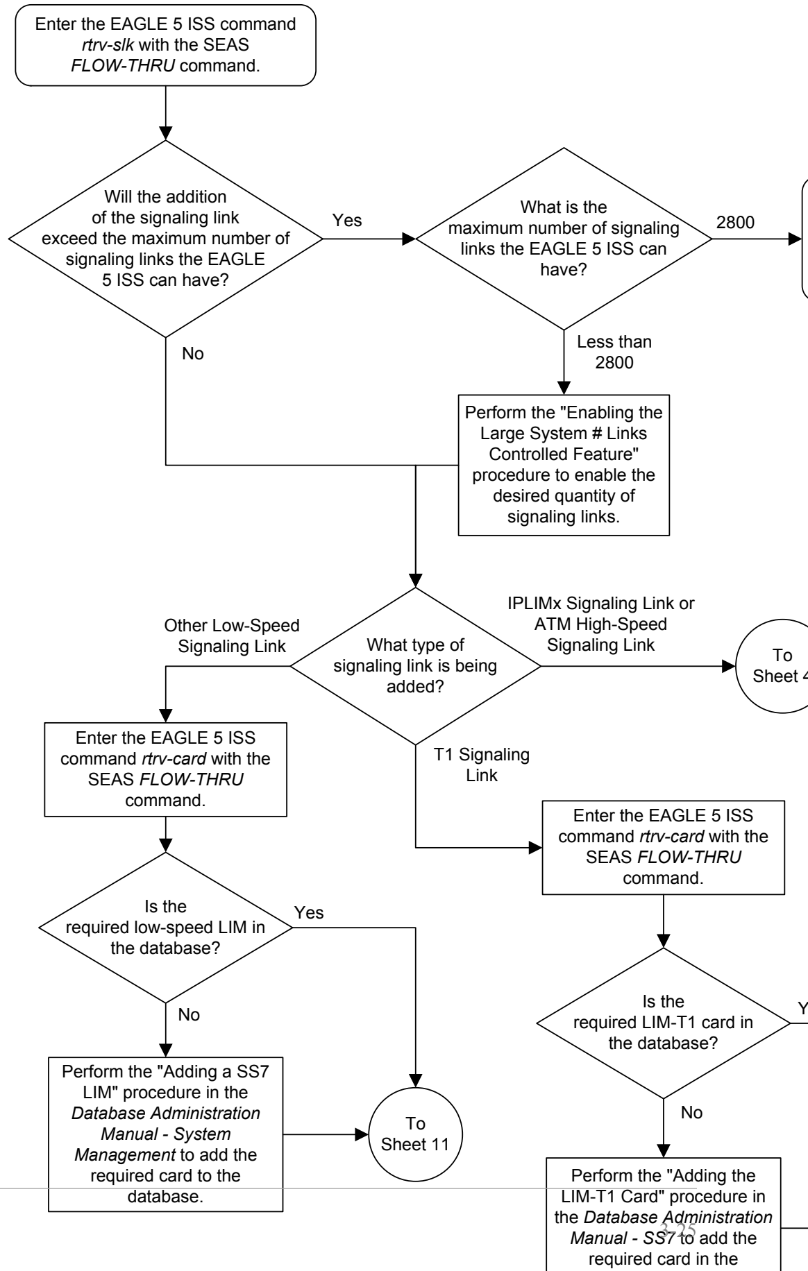
Figure 3-4 Adding an SS7 Signaling Link from the SEAS Terminal
