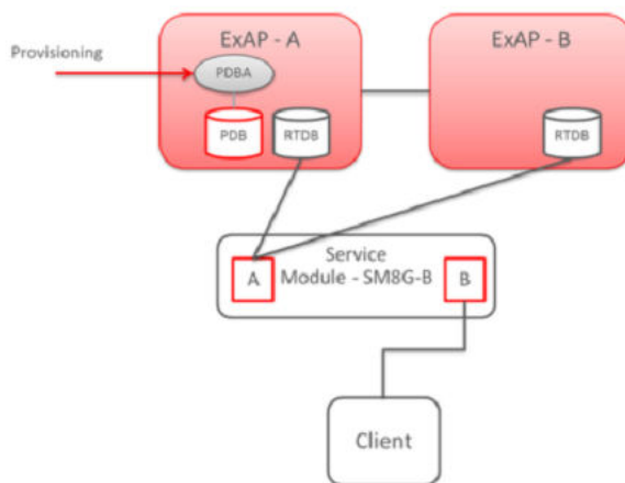
Figure 2-2 DEIR Network Connectivity without SLIC Card
