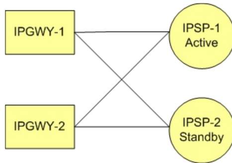
Figure A-2 IPGWx active/standby configuration
