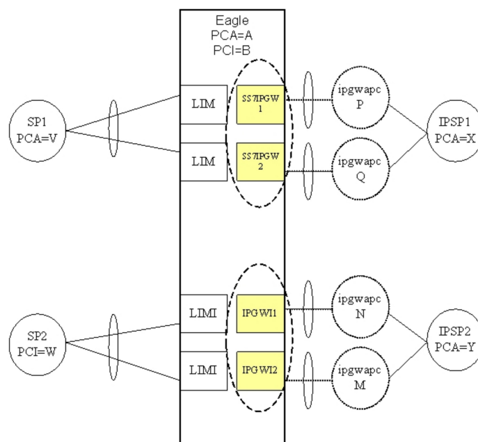
Figure A-3 Two-Pair IPGWx for maximum TPS
