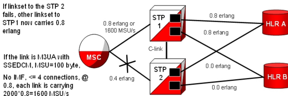
Figure 5-4 EAGLE: Failover at 0.8 Erlang and 1600 MSU/s
