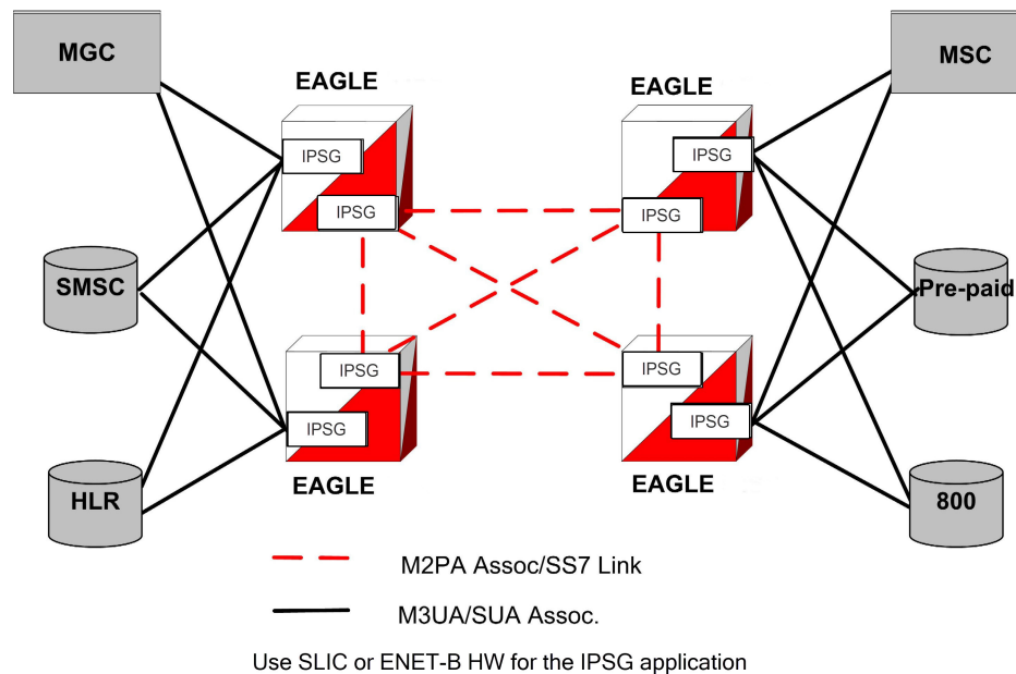
Figure 2-5 Typical EAGLE SS7-over-IP Deployment
