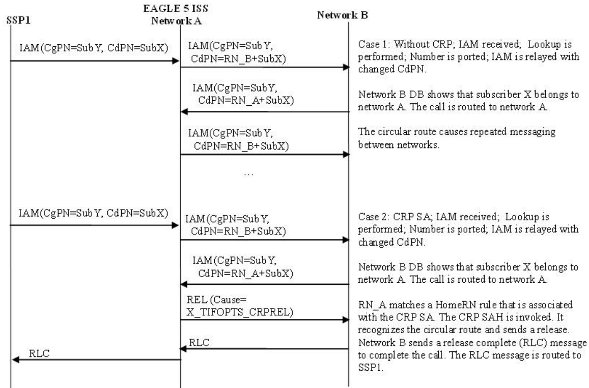
Figure 3-7 ISUP Message Flows for TIF CRP
