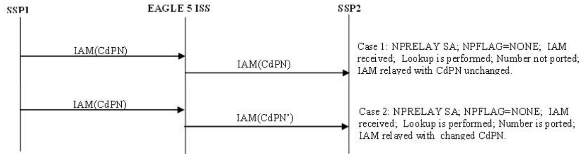
Figure 3-1 ISUP Message Flows for TIF NP CdPN Relay
