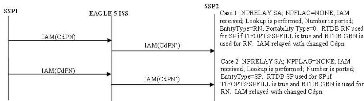
Figure 3-8 ISUP Message Flows for Service Portability
