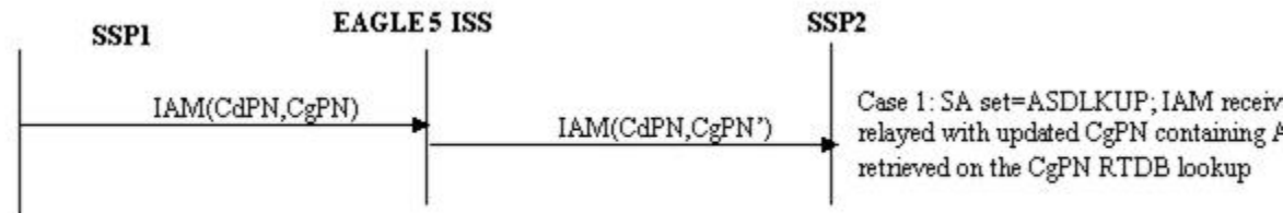
Figure 3-21 ISUP IAM Message Flow for TIF ASD for CgPN Service
