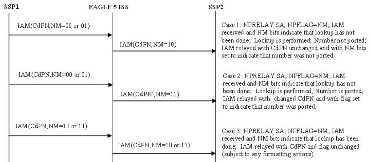
Figure 3-2 ISUP Message Flows for TIF NP CdPN Relay, with Optional NM Bits
