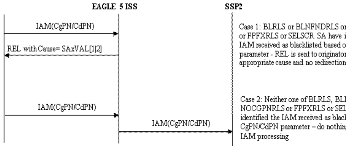
Figure 3-25 TIF Blacklist Basic Message Flow
