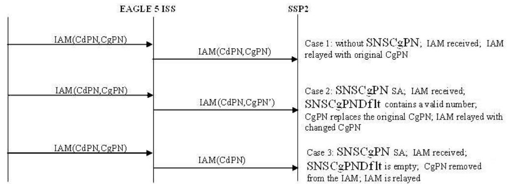
Figure 3-16 ISUP Message Flows for TIF SNS
