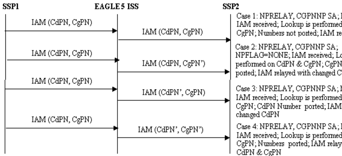
Figure 3-4 ISUP Message Flows for TIF NP CgPN with NPRELAY and CGPNNP
