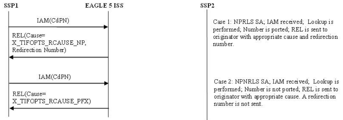
Figure 3-5 ISUP Message Flows for TIF NP Release
