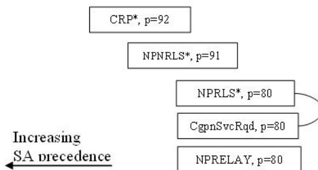
Figure 3-10 NP Service Action Precedence
