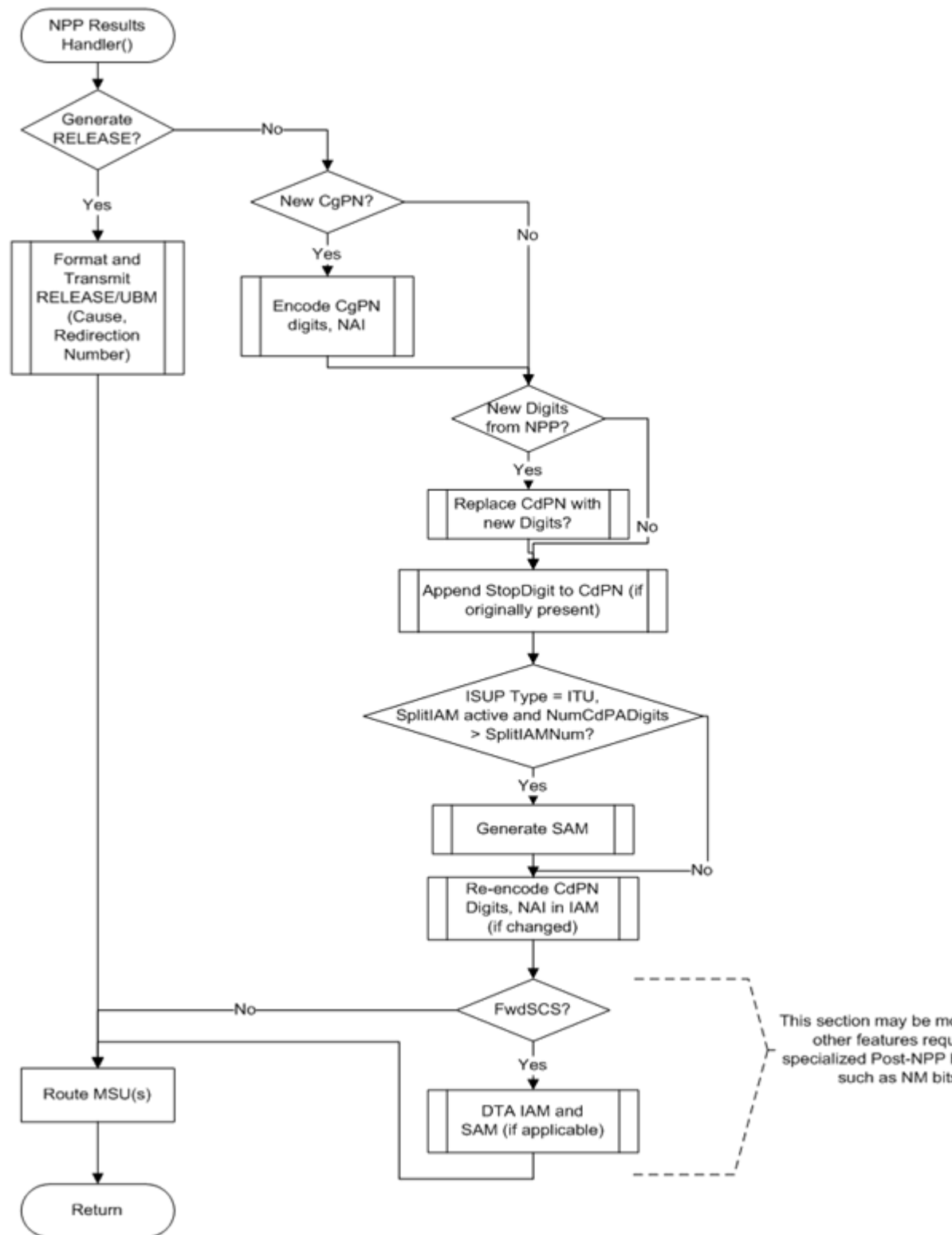
Figure 2-6 TIF Post-NPP Results Handler
