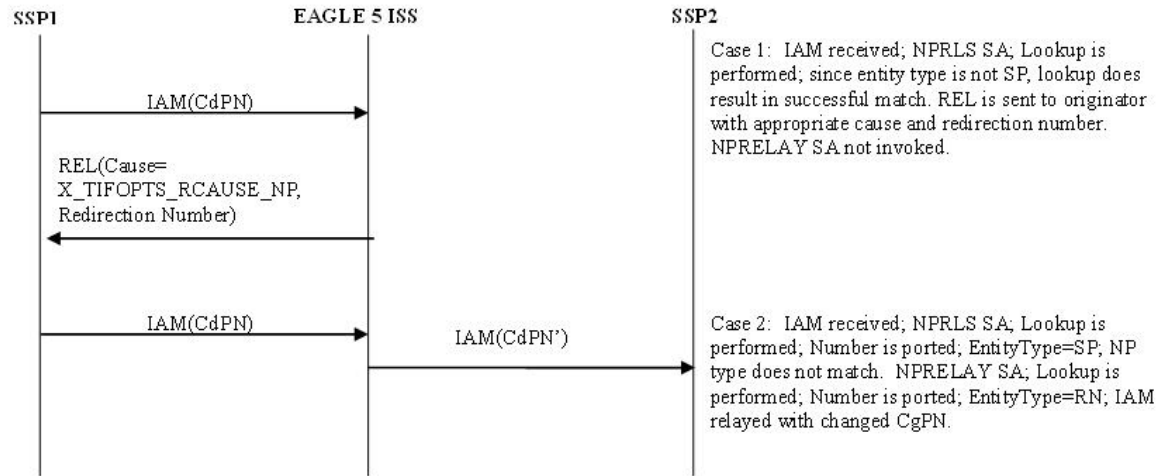
Figure 3-9 ISUP Message Flows for NPRLS + NPRELAY
