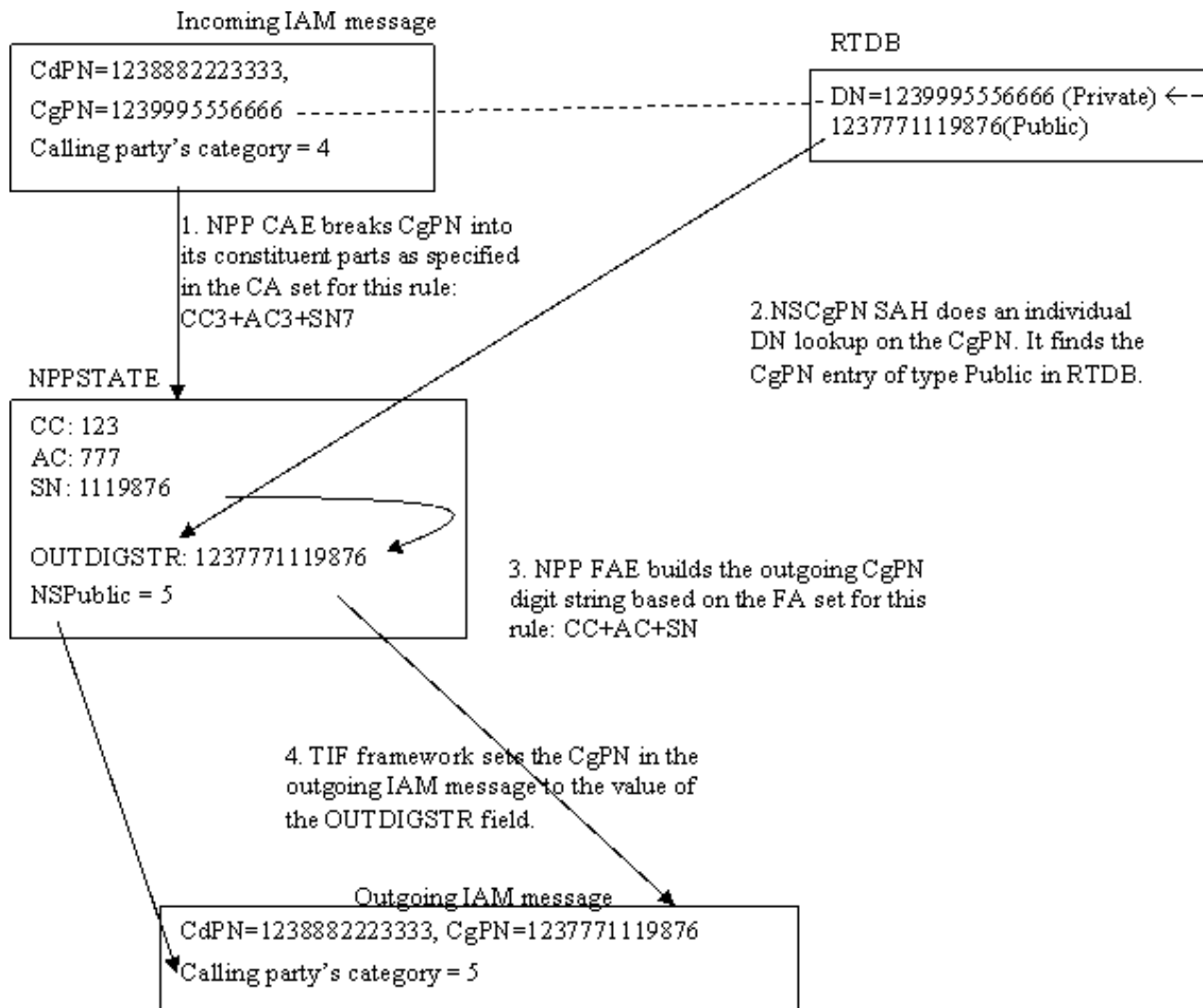
Figure 3-15 TIF NS Basic Operation for TIF CgPN Service
