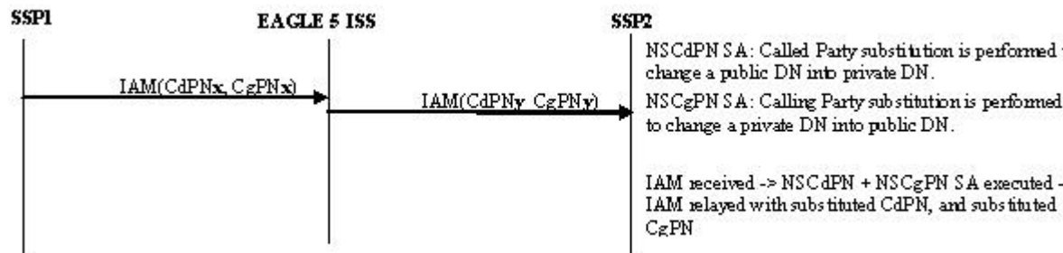
Figure 3-11 ISUP RELAY with TIF NS
