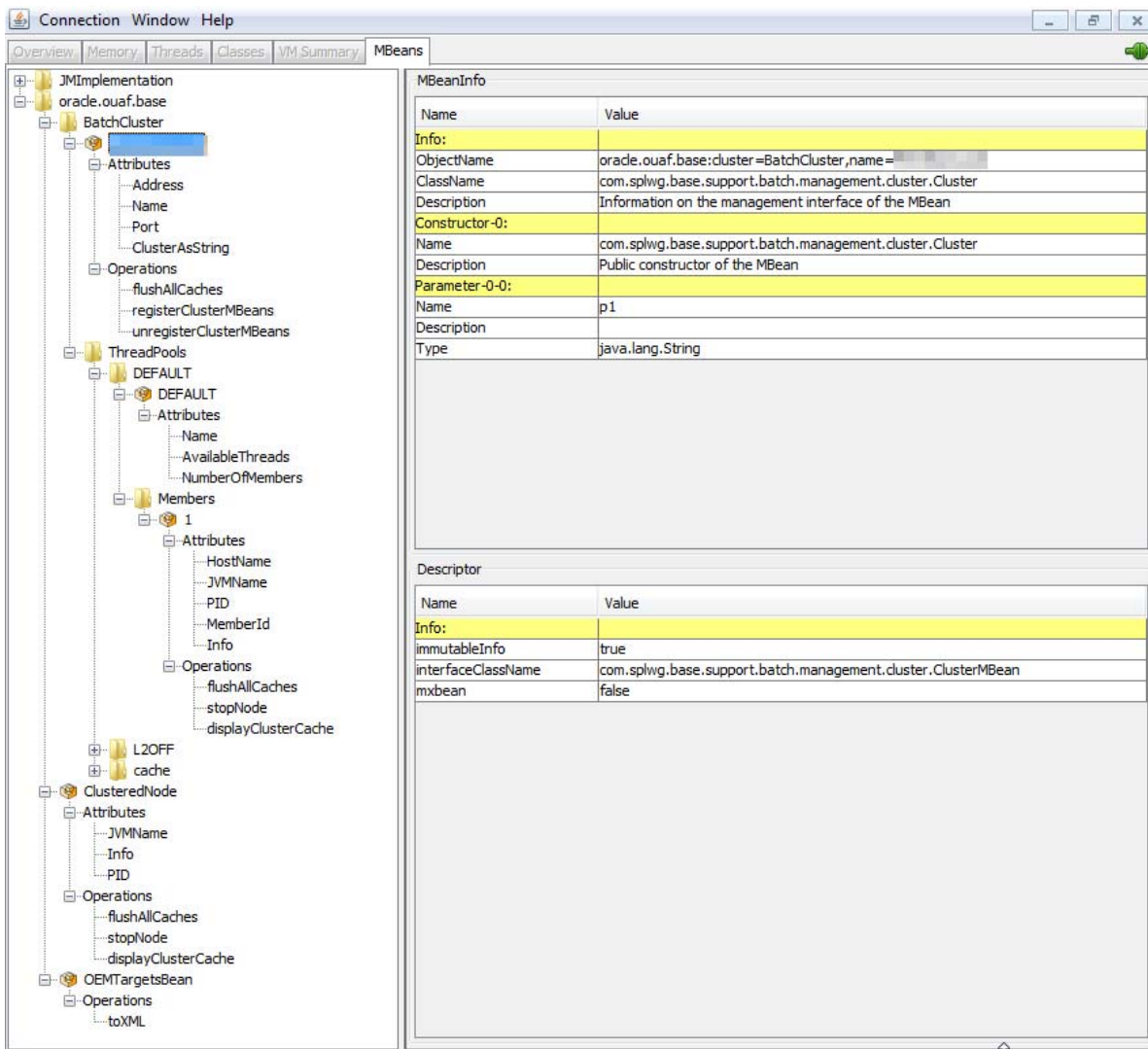
Figure 11 – Example Batch Server Mbeans in jconsole
