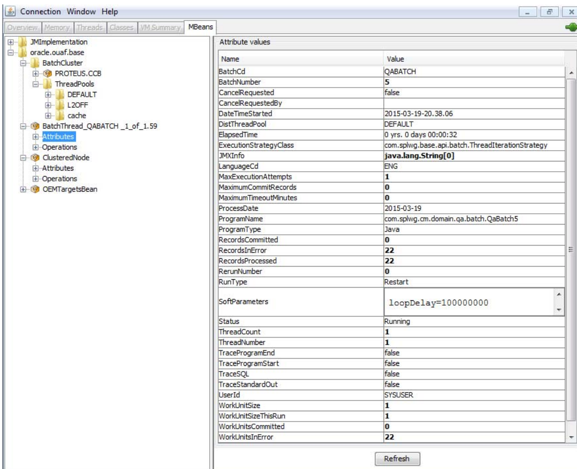
Figure 12 – Example Batch Thread Mbean in jconsole
