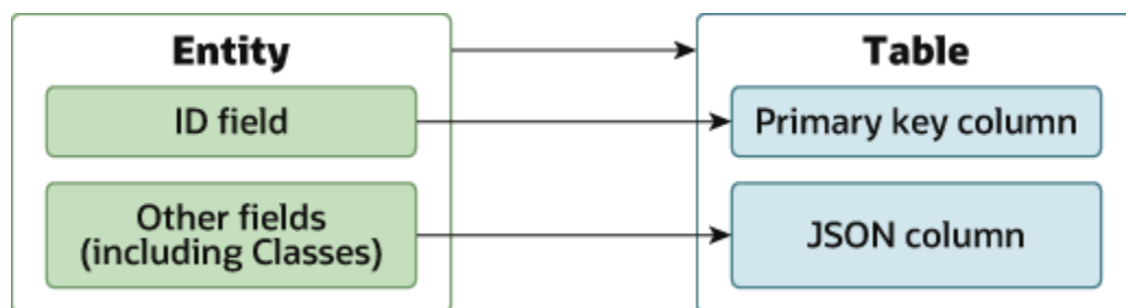
Figure 1-2 Persistence Model
