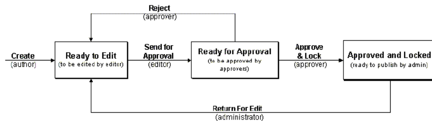
Figure 9-2 Workflow-Flowchart
