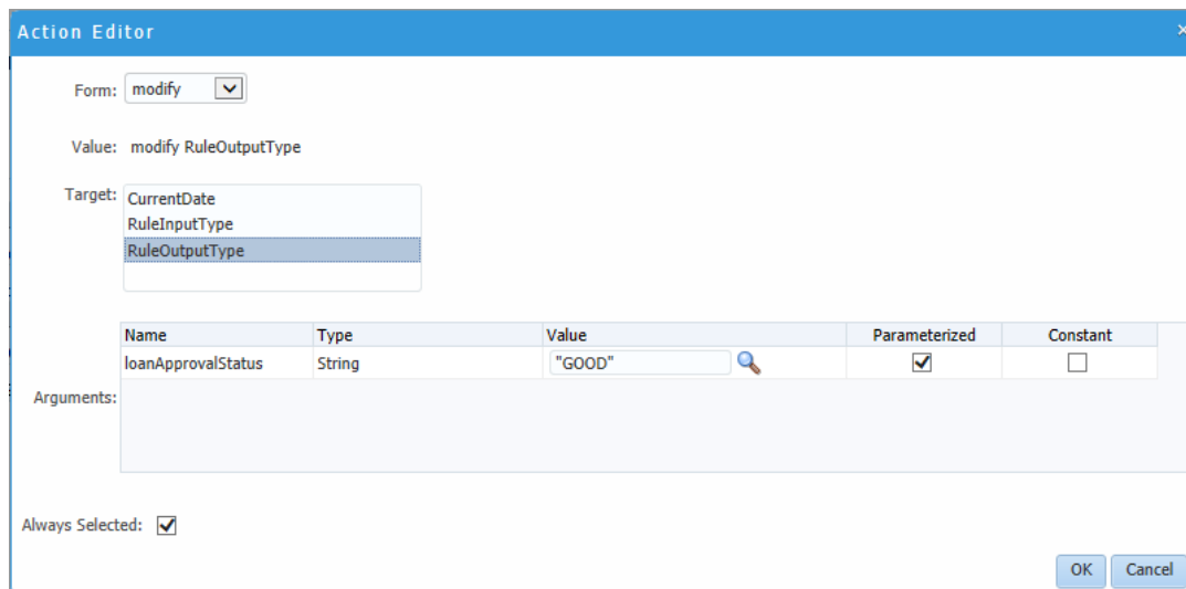
Figure 17-11 Action Editor Showing Parameterized Action with Default Value
