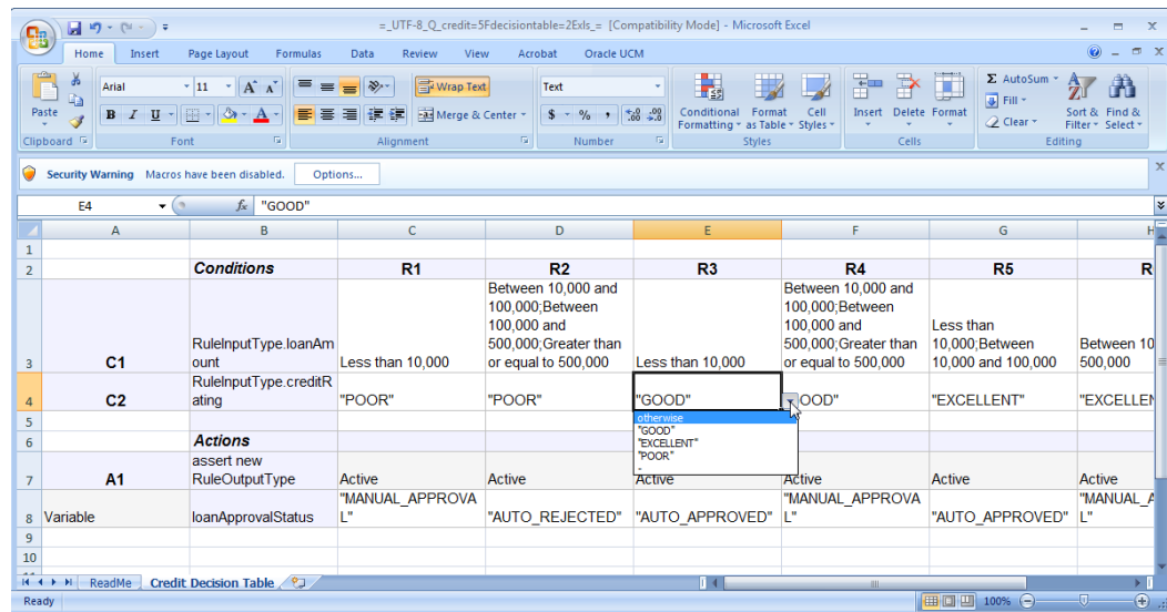
Figure 17-13 Microsoft Excel - Decision Table
