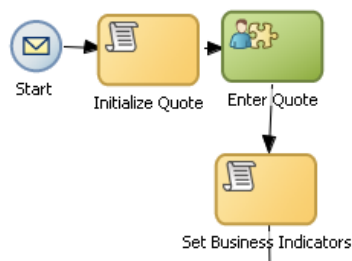
Figure A-14 The Enter Quote User Task
