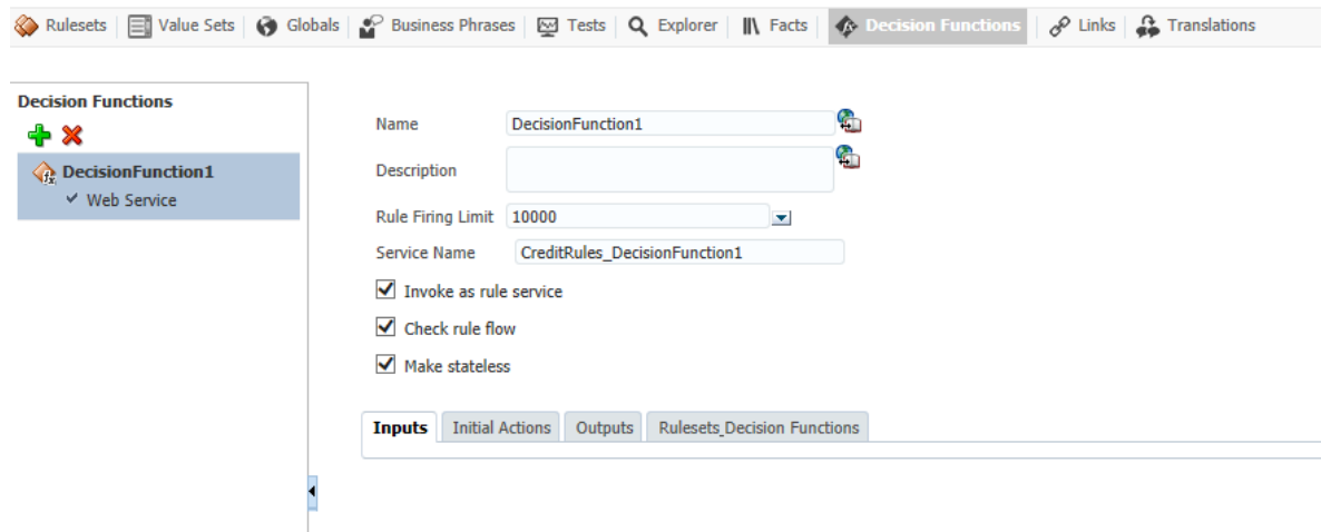
Figure 17-20 Business Rules Editor - Decision Functions
