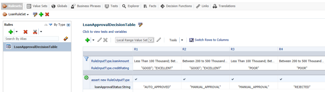
Figure 17-12 Business Rules Editor: Rulesets - New Decision Table Rule
