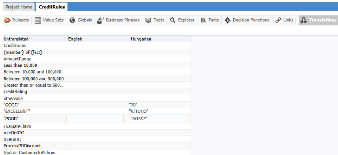
Figure 17-23 Business Rules Editor - Translations
