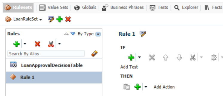
Figure 17-8 Business Rules Editor: Rulesets - New General Rule
