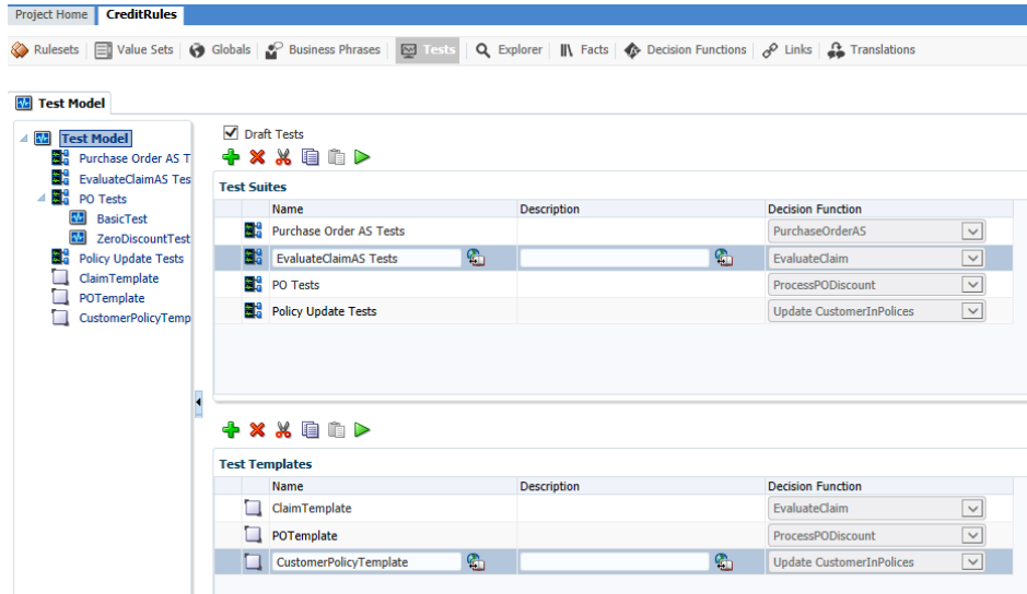
Figure 17-21 Business Rules Editor - Tests
