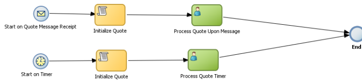
Figure A-1 Using Multiple Start Events within a Process
