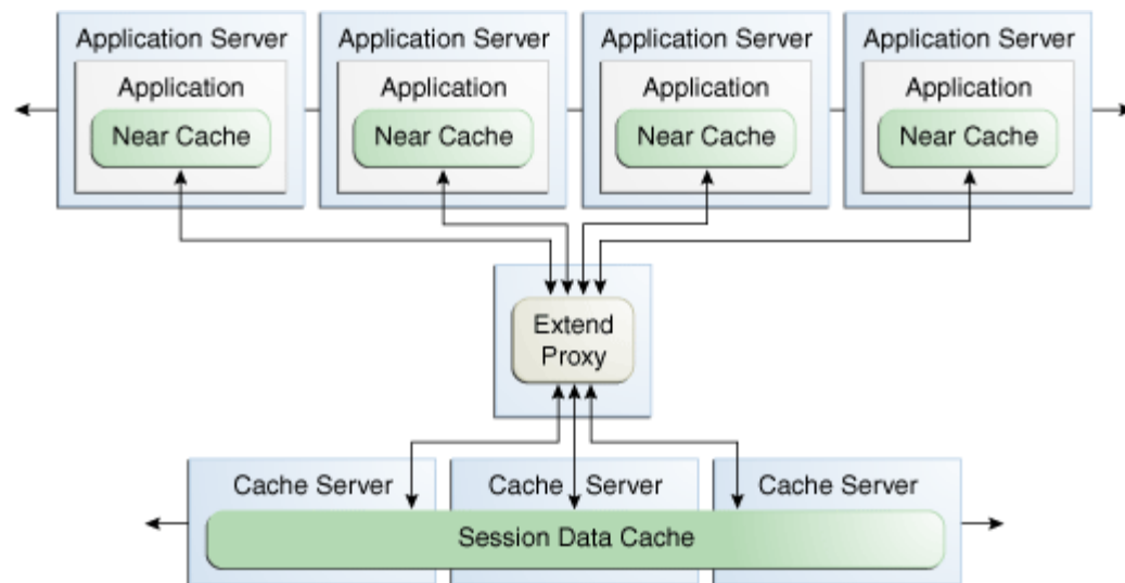
Figure 5–11 Out-of-Process with Coherence*Extend Deployment Topology
