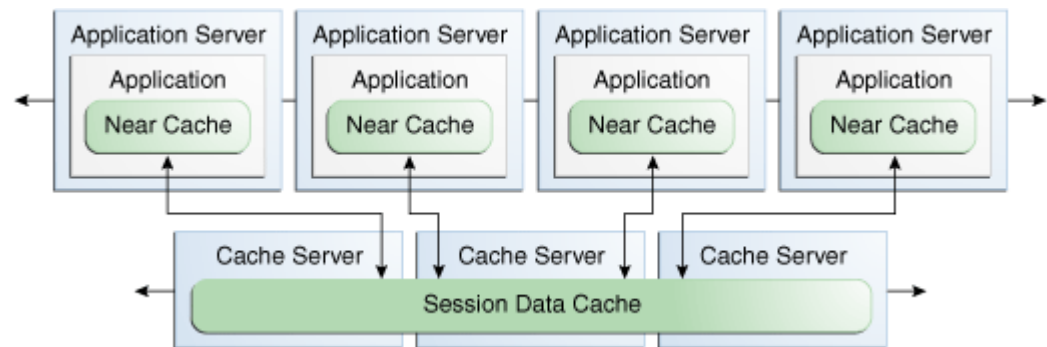
Figure 5–10 Out-of-Process Deployment Topology
