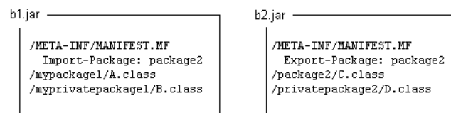
Figure 6-1 Example Oracle Event Processing Event Processing Applications
