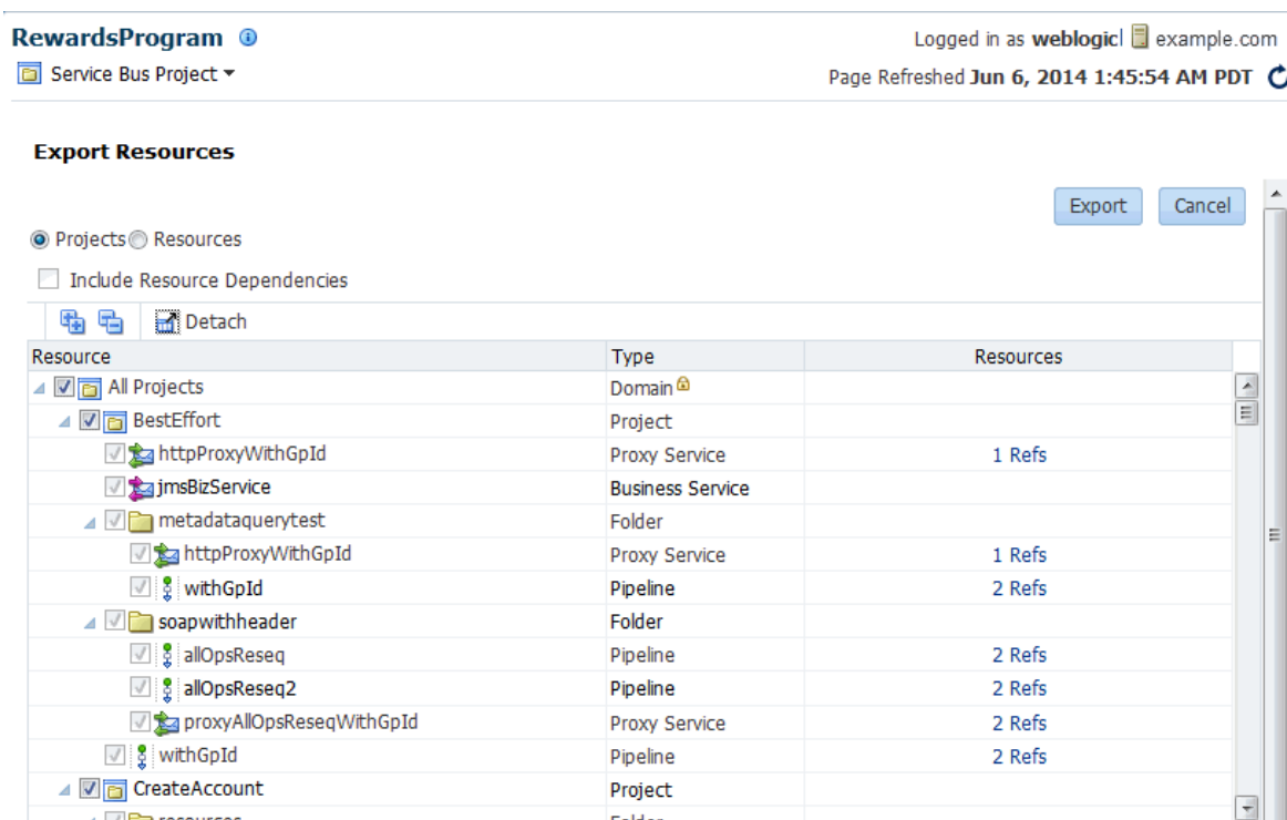
Figure 10-1 Export Resources Page
