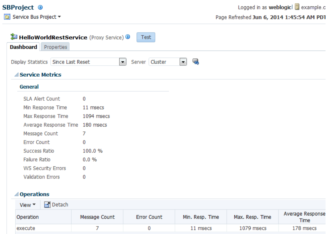
Figure 5-2 Service Bus Service Dashboard
