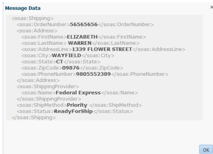
Figure 12-6 Message Report Data
