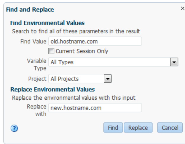
Figure 9-2 Find and Replace Dialog with Replacement Value
