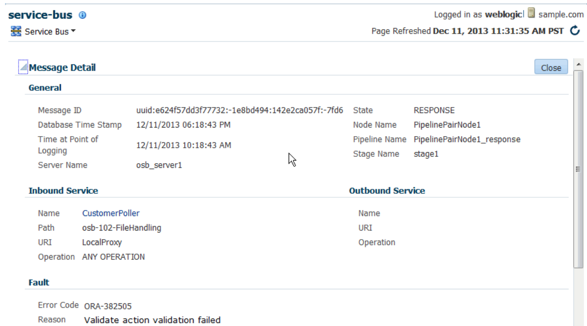
Figure 12-5 Message Reports Message Detail Window
