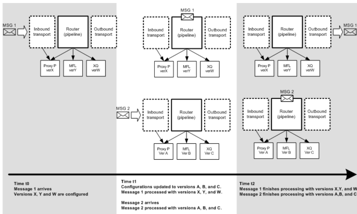
Figure 59-1 Sample Online Update Scenario
