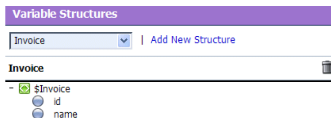
Figure 13-6 Variable Structures—Invoice
