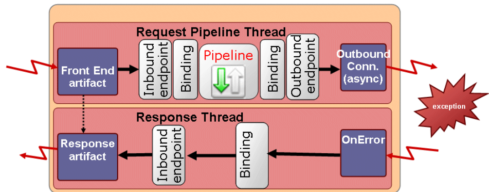
Figure 40-3 Error Case 2
