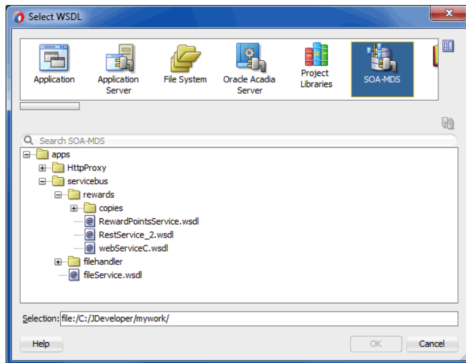
Figure 45-6 Resource Browser
