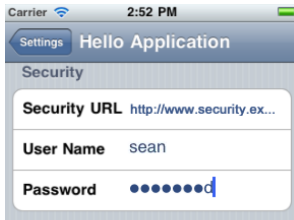
Figure 22-18 Text Preferences
