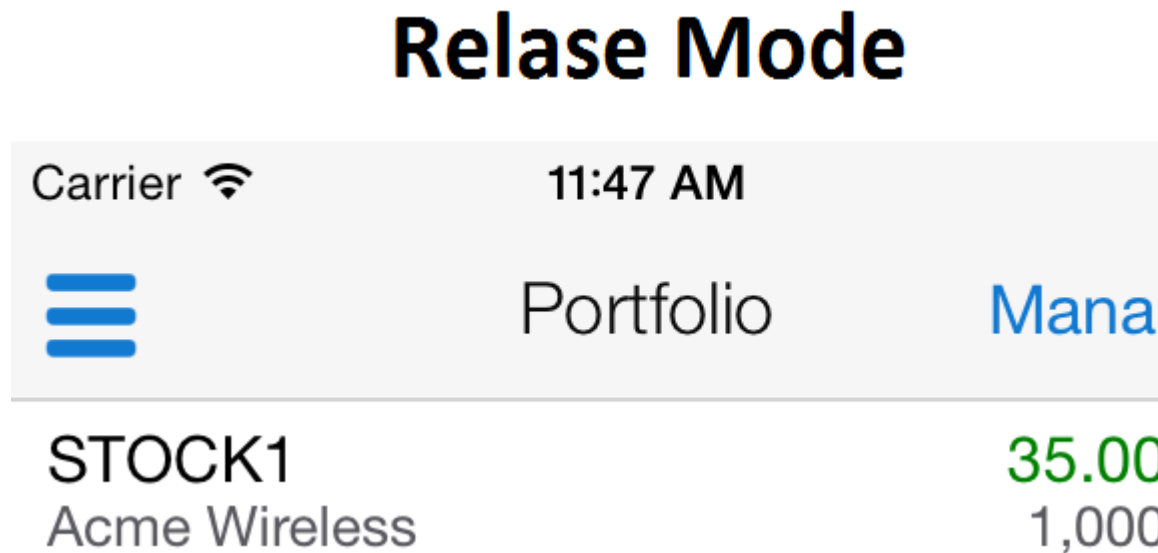
Figure 27-9 Deployment Modes
