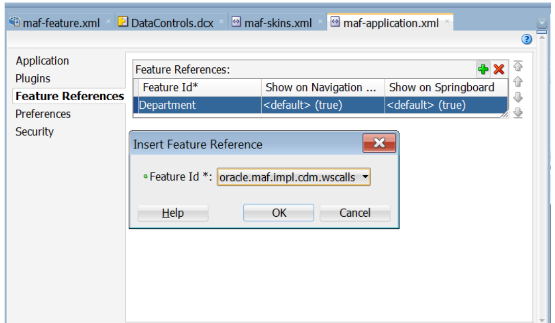
Figure 30-17 maf-application.xml file
