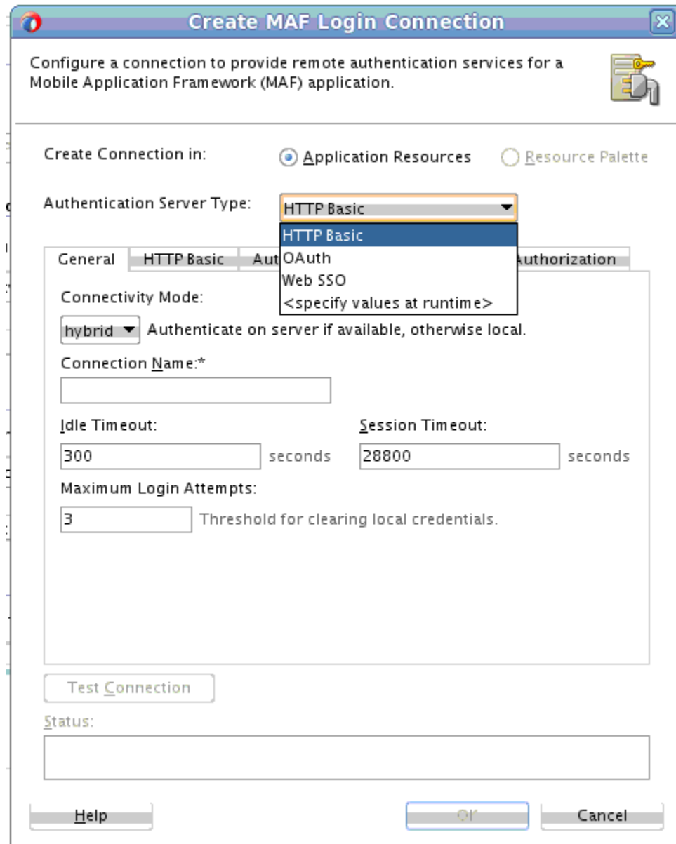
Figure 29-2 Configuring Authentication
