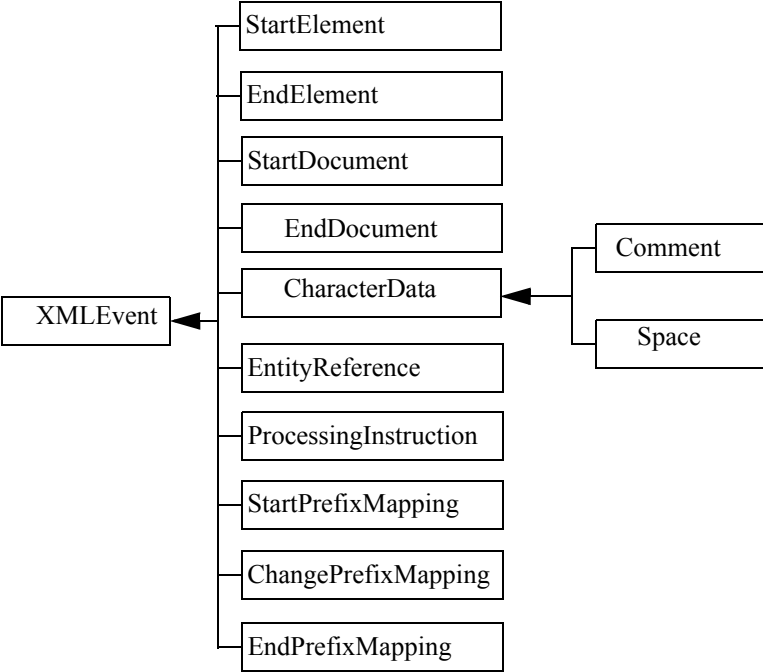
Figure 9-1 Hierarchy of the XMLEvent Interface and Its SubInterfaces
