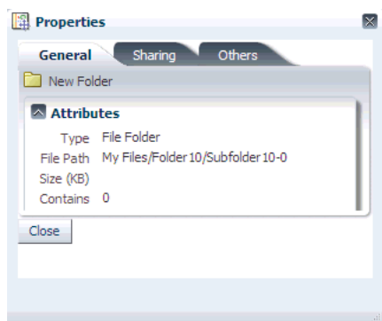
Figure 13–1 af:dialog Component
