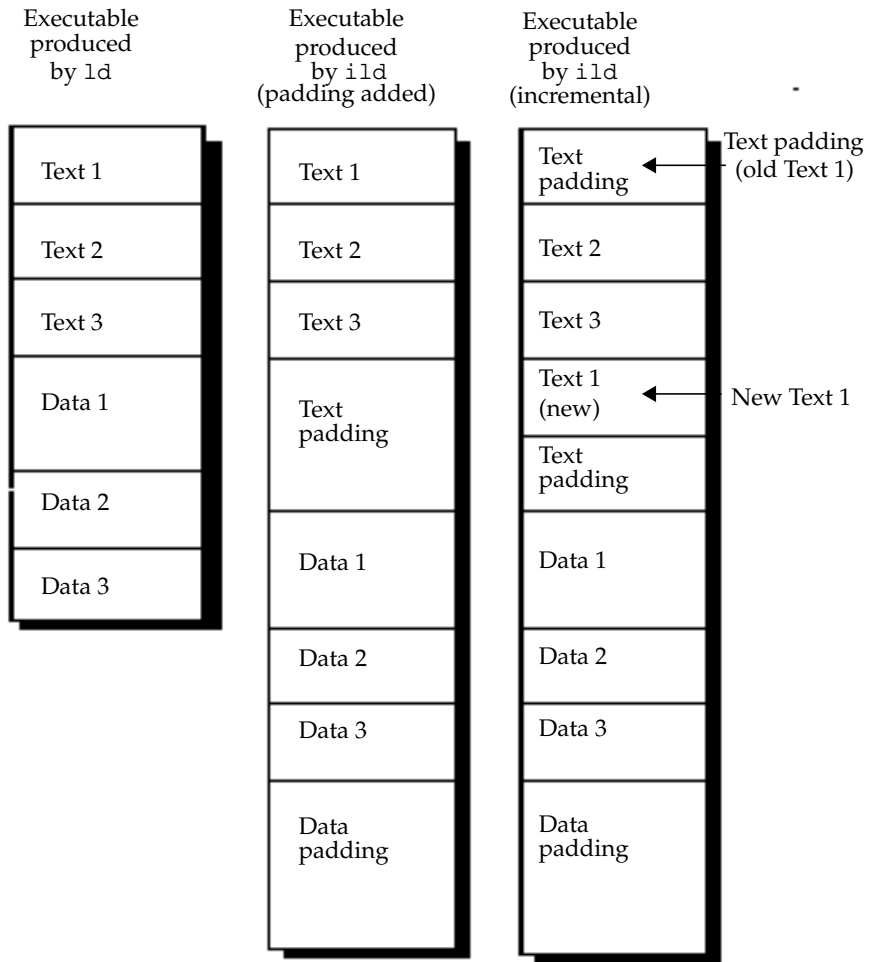
FIGURE 5-1 An Example of Incremental Linking
