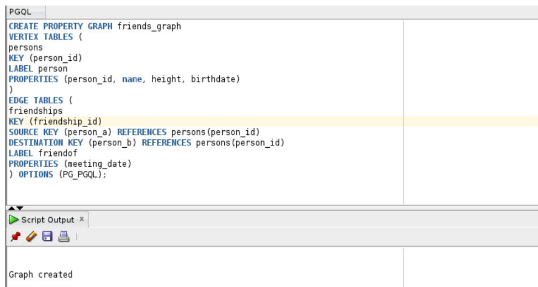
Figure 16-5 Create a PGQL property graph
