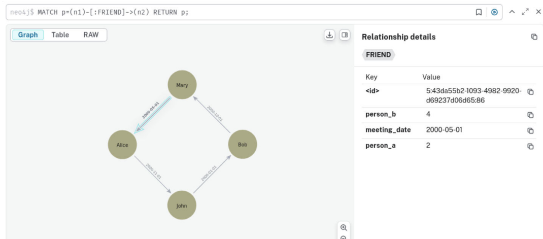
Figure 4-3 Example Graph in Neo4j for Migration
