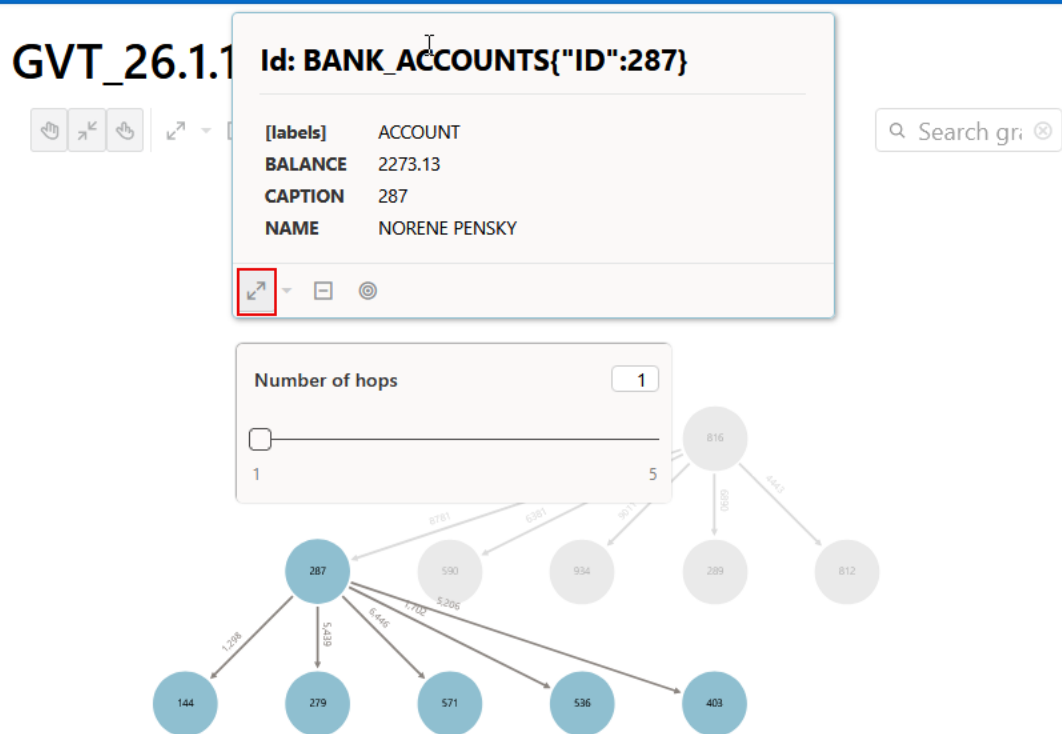
Figure 9-18 Expanding on a Specific Graph Vertex
