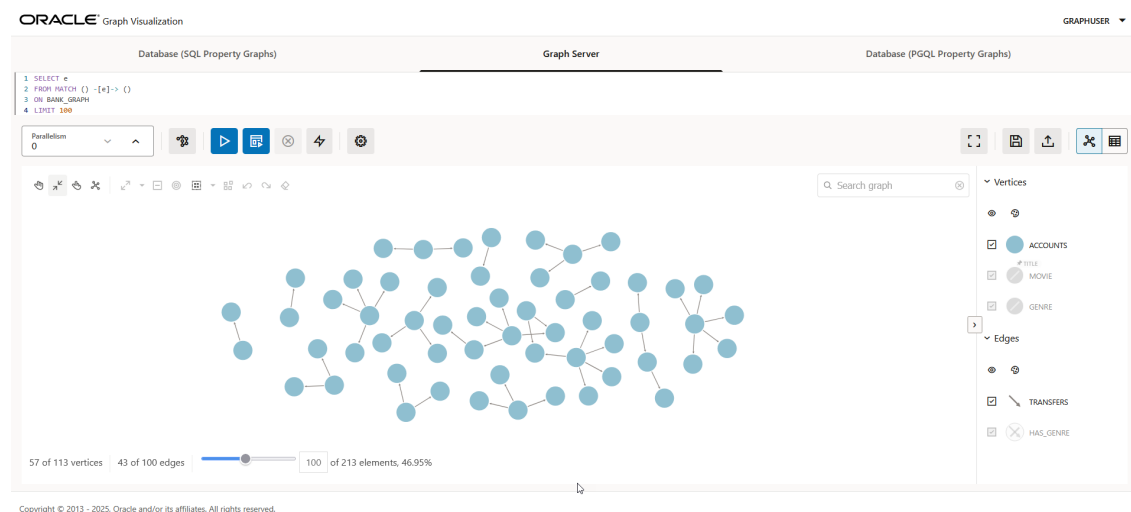
Figure 25-8 Visualizing a PGQL Query
