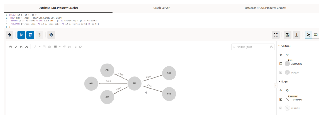
Figure 4-2 Visualizing a SQL Graph Query
