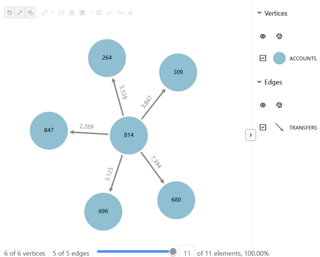
Figure 9-1 Visualizing a SQL Graph Query in an APEX Application
