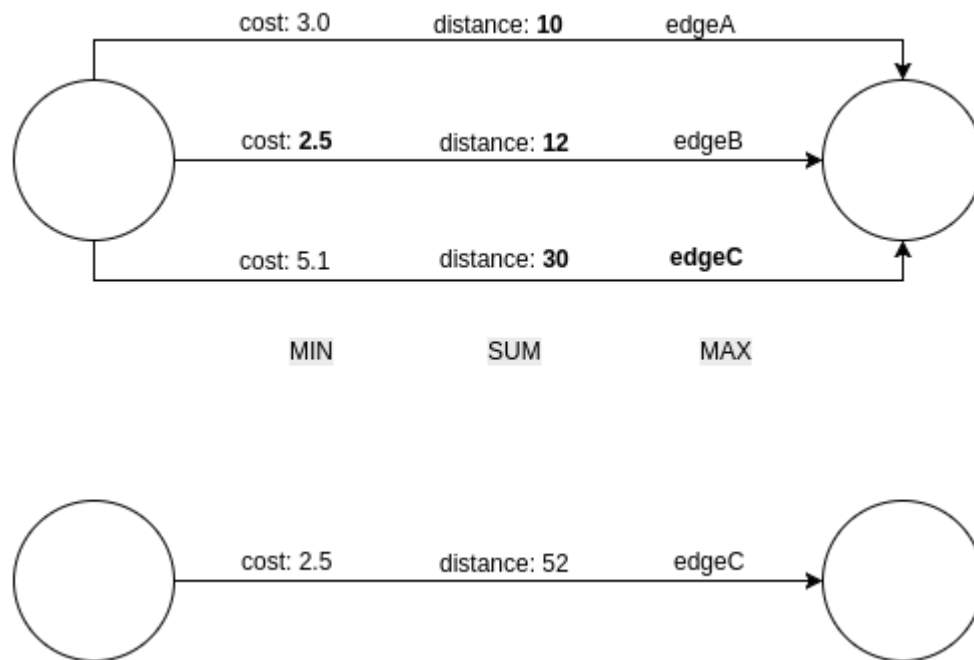
Figure 31-2 Merging Strategy
