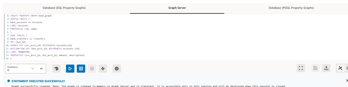
Figure 25-4 Creating a Property Graph in the Graph Server Memory
