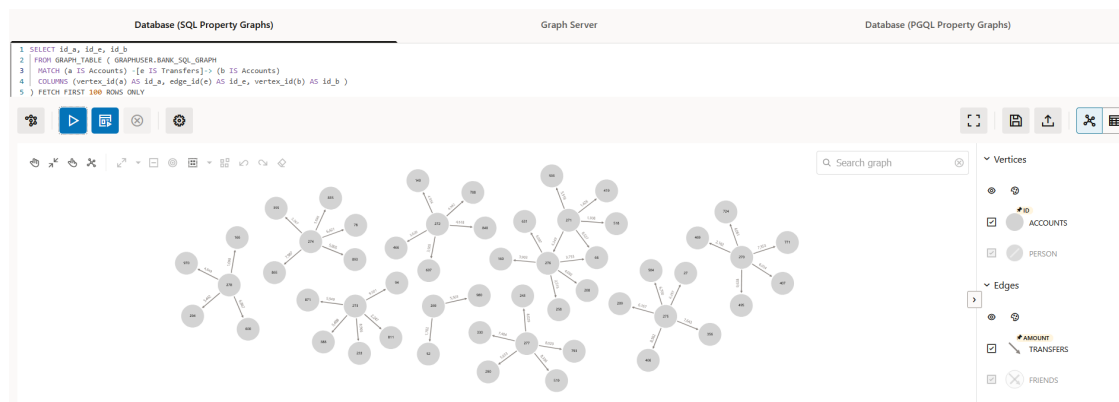
Figure 25-3 Graph Query on a SQL Property Graph
