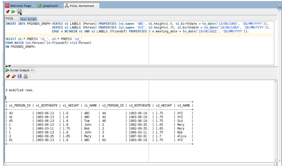
Figure 16-6 Running Multiple PGQL Queries
