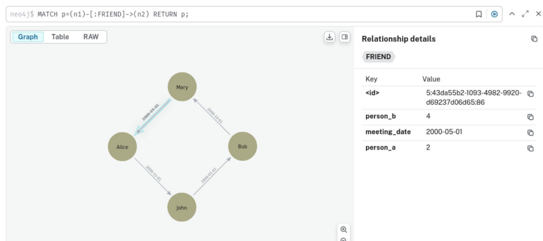
Figure 4-4 Example Graph in Neo4j for Migration
