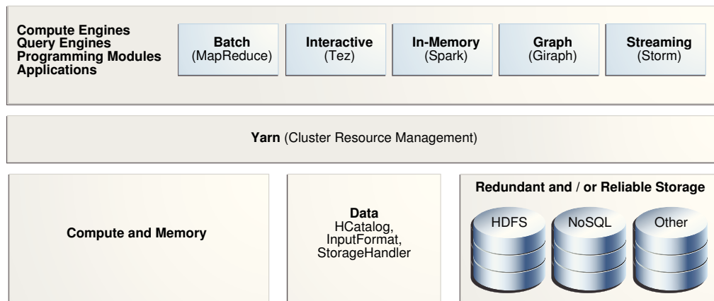
Figure 6-1 Hadoop 2.0 Architecture
