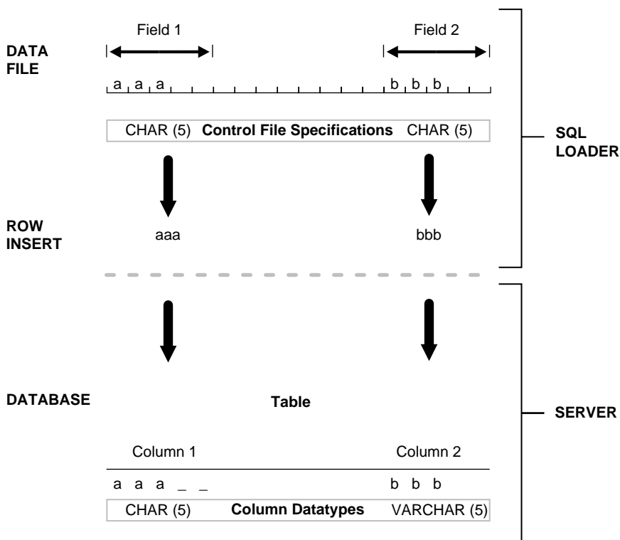
Figure 3-3 Example of Field Conversion
