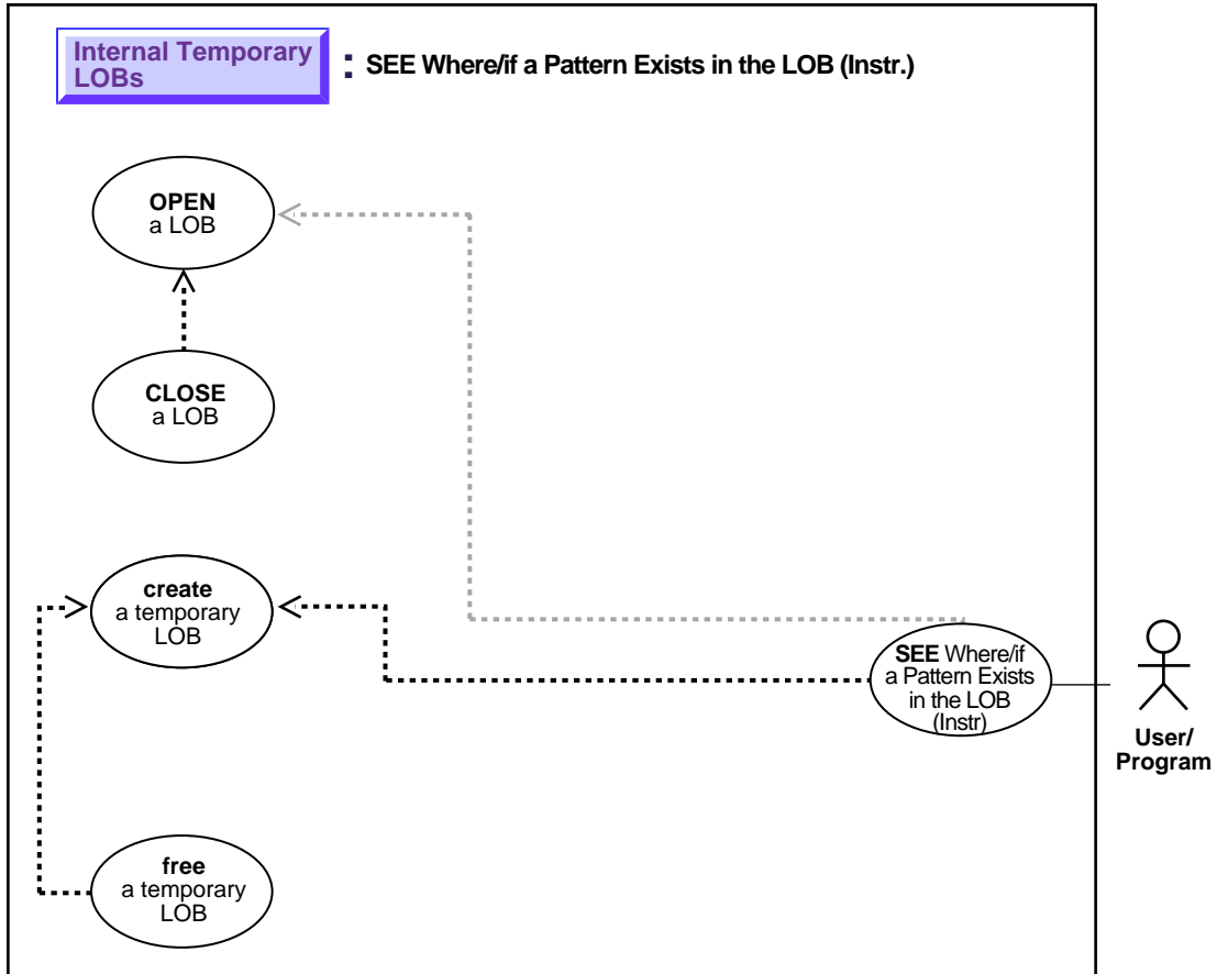
Figure 10–12 Use Case Diagram: See If a Pattern Exists in a Temporary LOB (instr)
