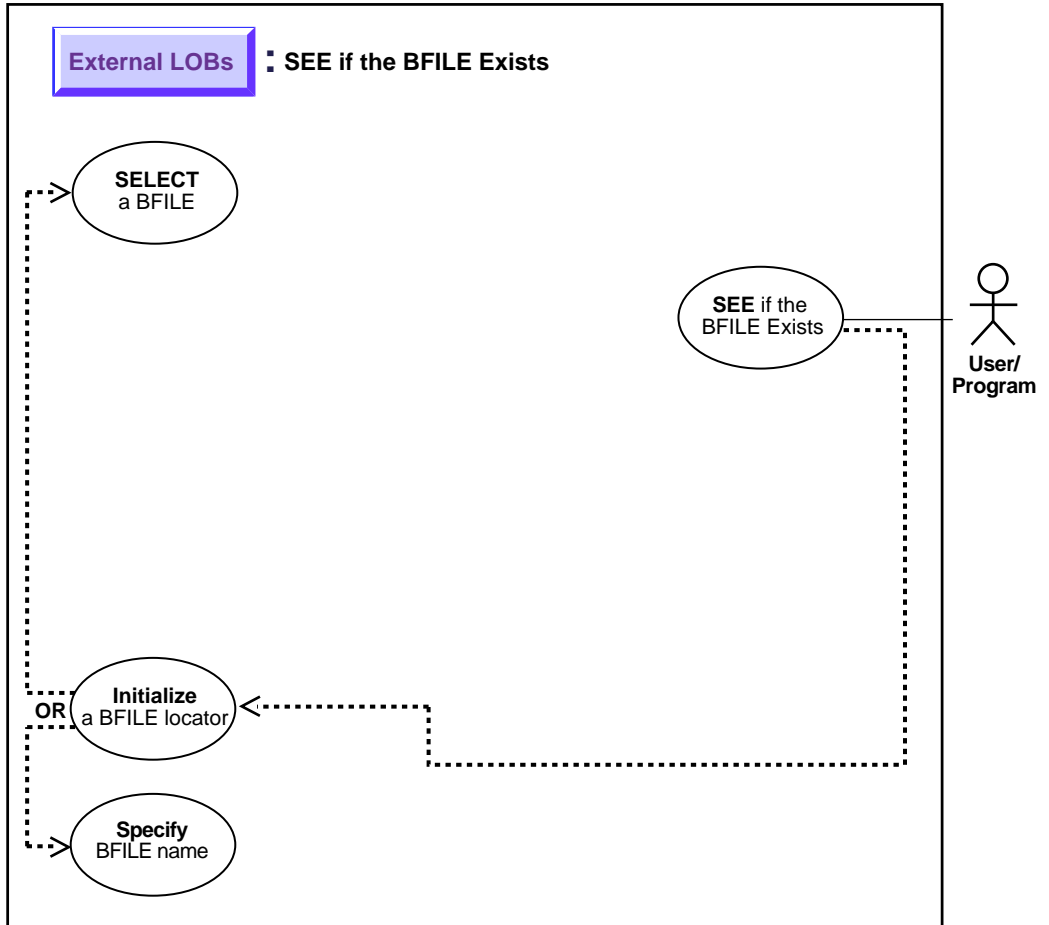
Figure 11–23 Use Case Diagram: See If the BFILE Exists
