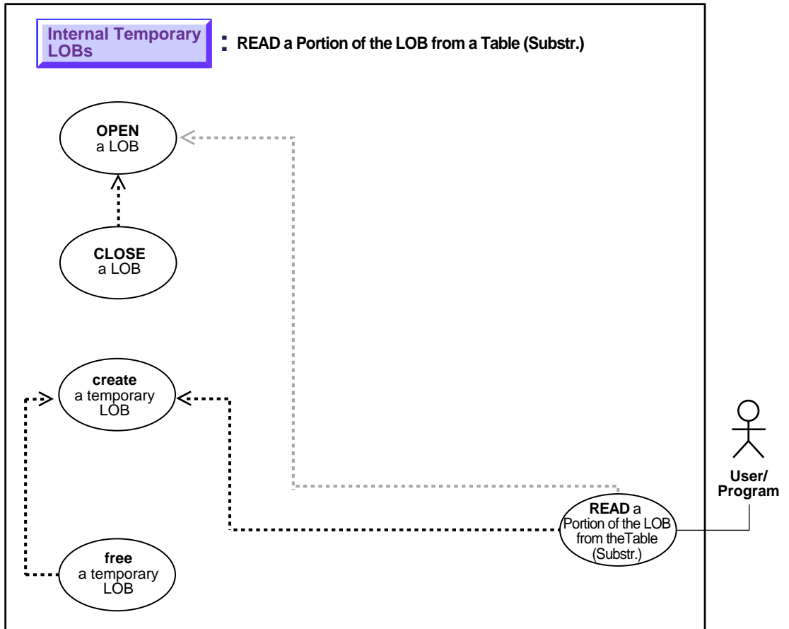
Figure 10–10 Use Case Diagram: Read Portion of Temporary LOB from the Table (substr)
