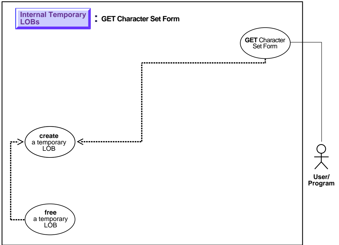
Figure 10–19 Use Case Diagram: Get Character Set Form of a Temporary LOB
