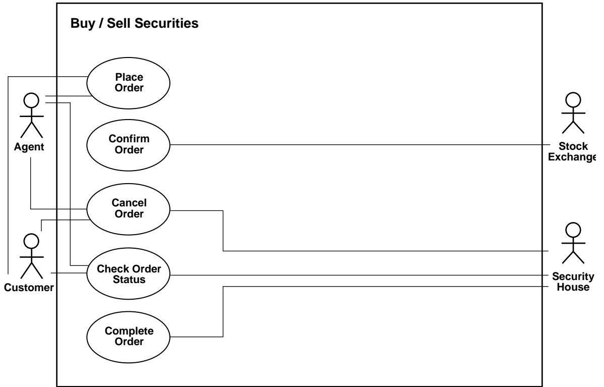
Figure 0-3 Use Cases
