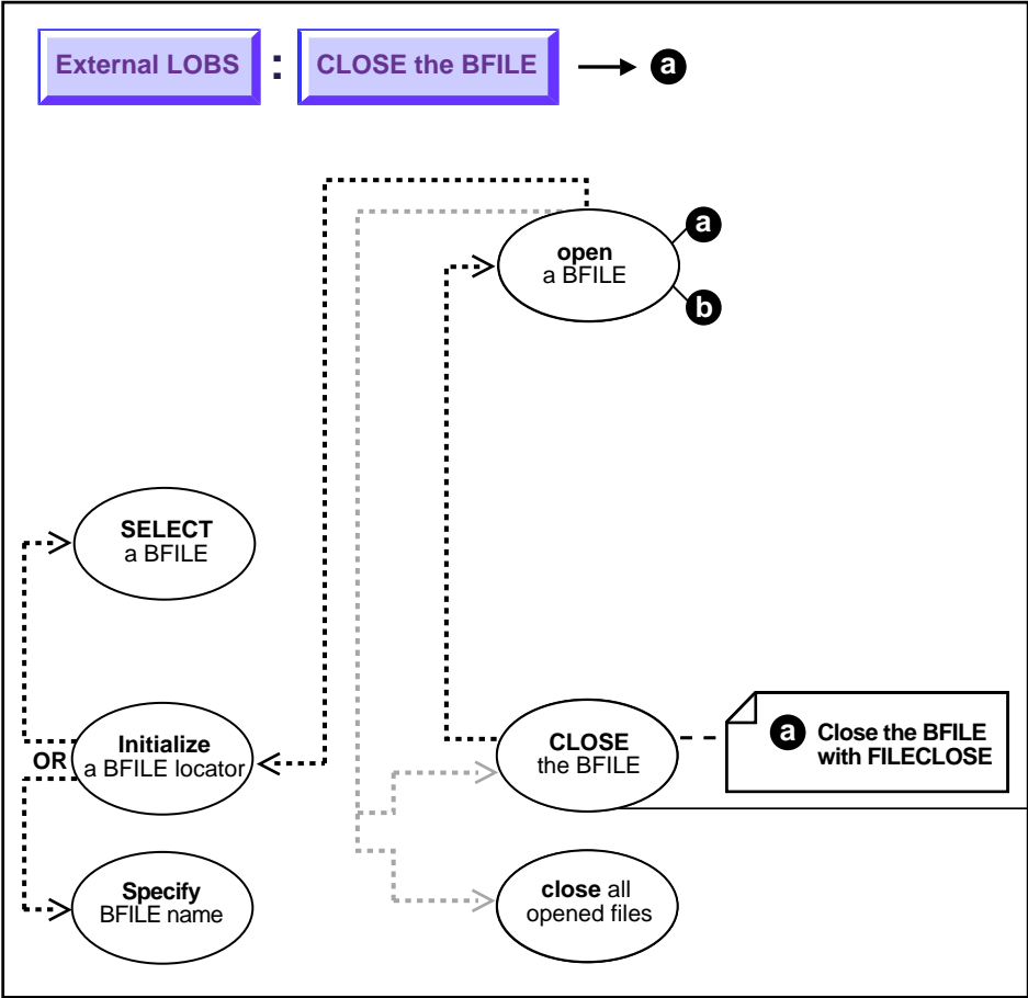
Figure 11-34 Use Case Diagram: Close a BFILE with FILECLOSE
