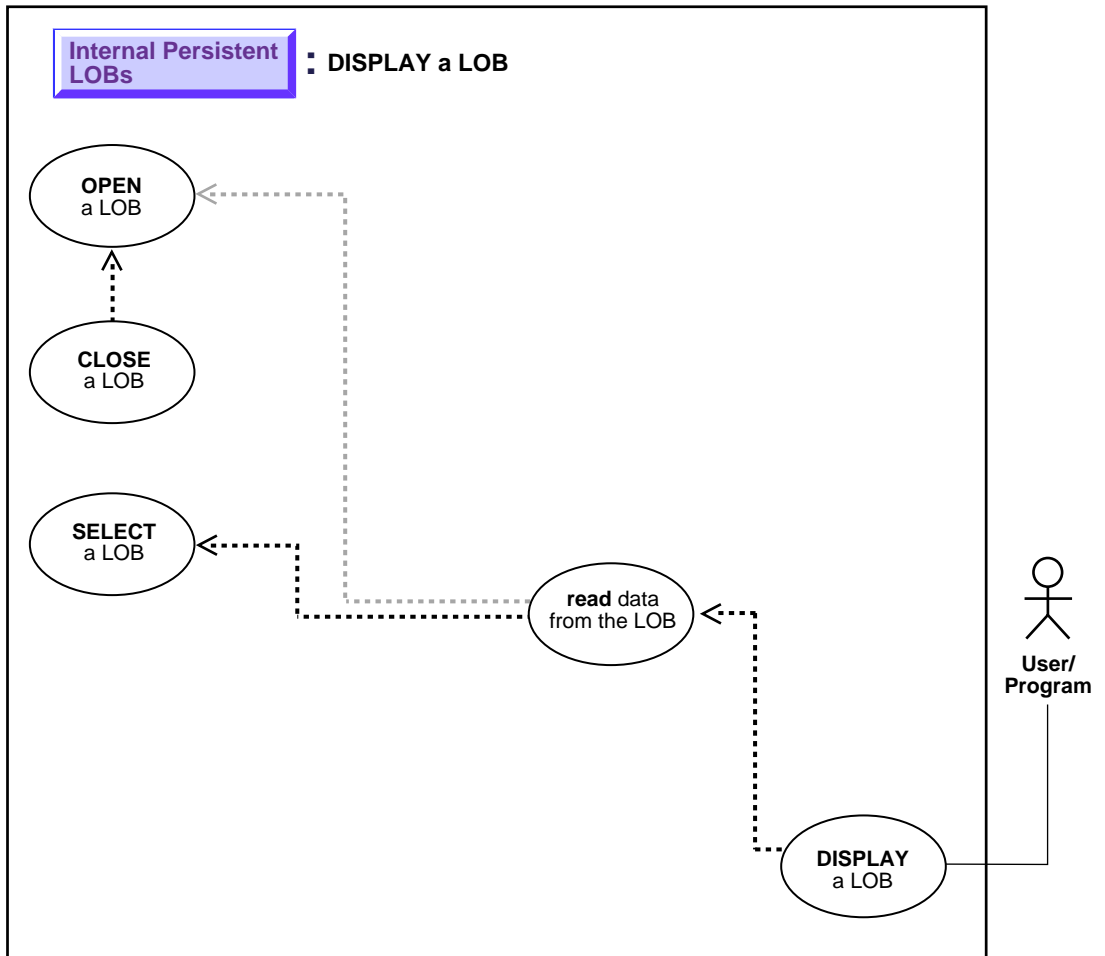
Figure 9-21 Use Case Diagram: Display LOB Data
