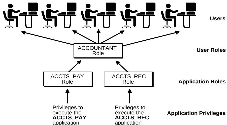
Figure 19–1 User Role
