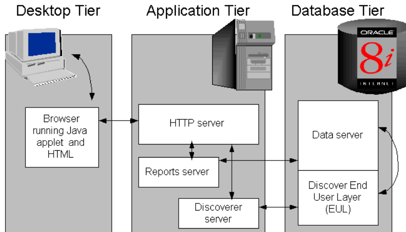
Figure 1–4 BIS Architecture
