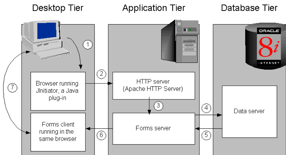
Figure 1–2 Forms-based Architecture
