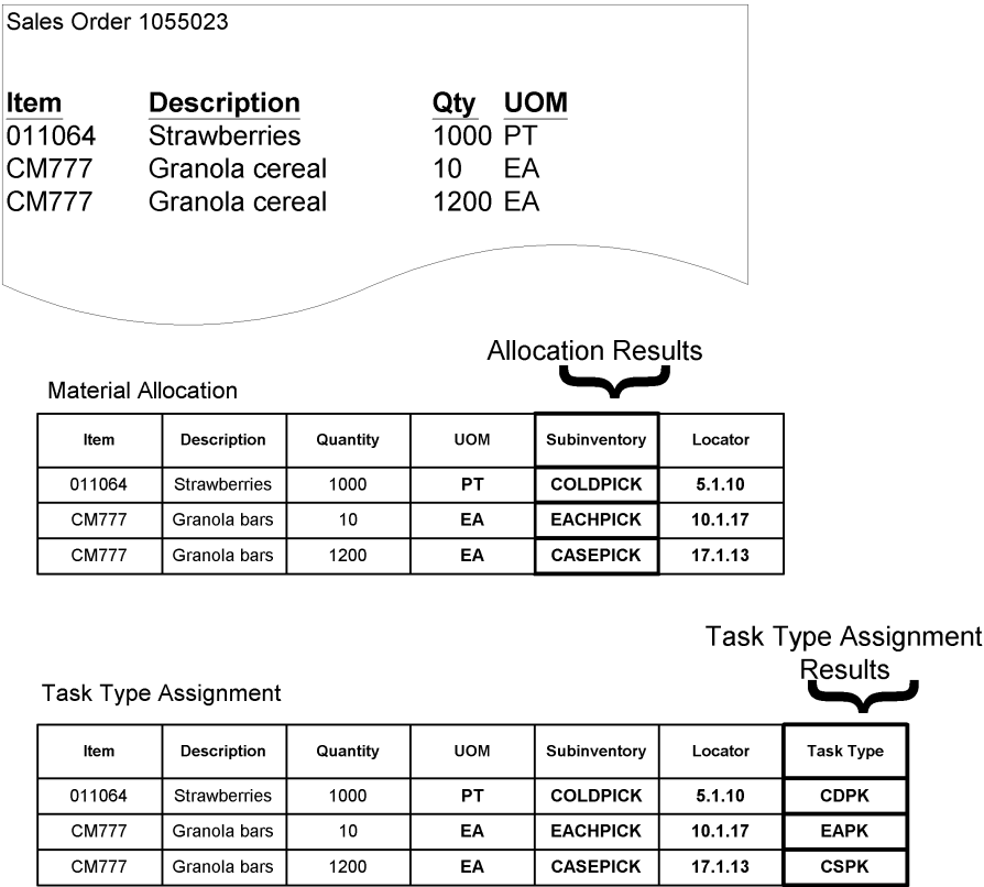
Figure 4–27 Material Allocation Example
