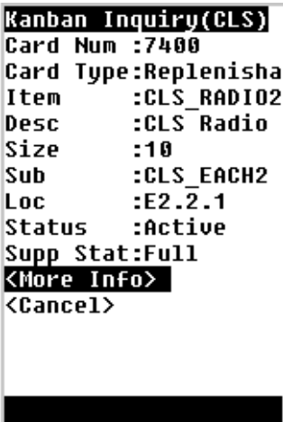
Figure 4–26 Mobile User Interface - Kanban Inquiry
