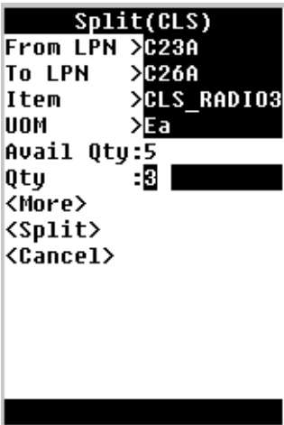
Figure 6–4 Mobile User Interface - Splitting Form
