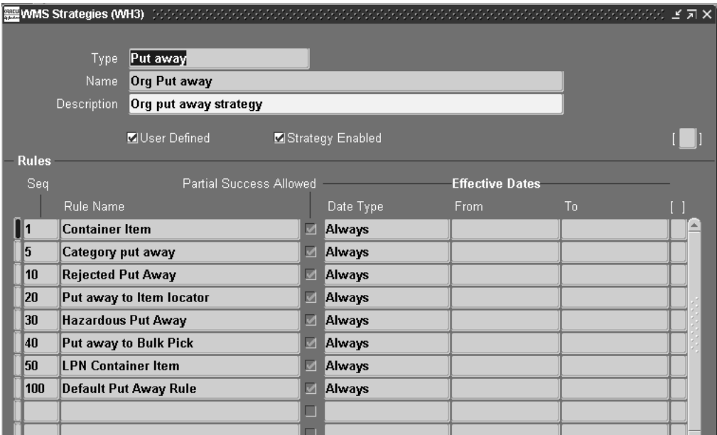
WMS Strategies Window
