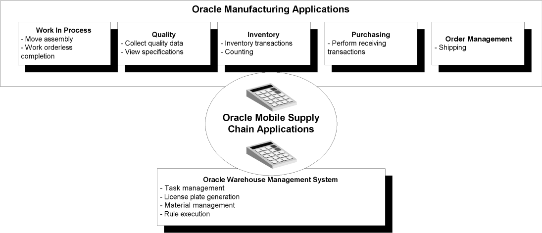
Figure B–1 Mobile Supply Chain Applications Integration
