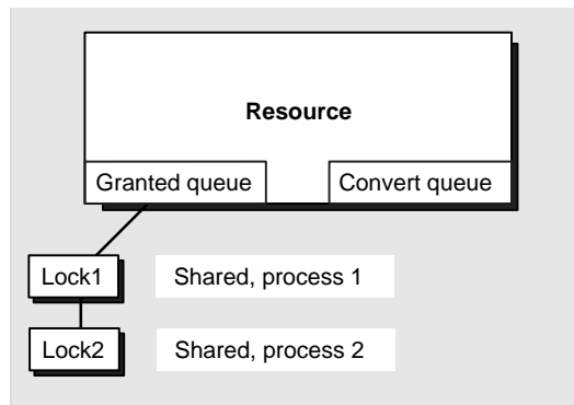
Figure 5-5 The Global Cache Service Grants and Converts Queues
