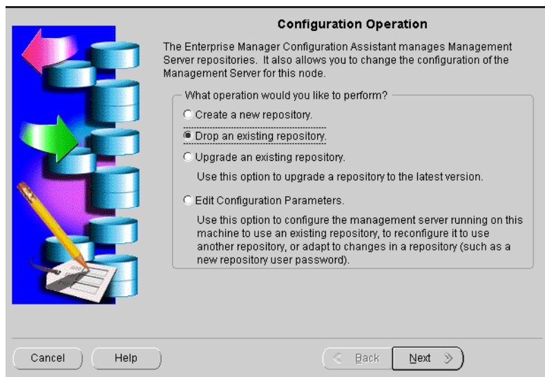
Figure 8–2 Configuration Operation Screen
