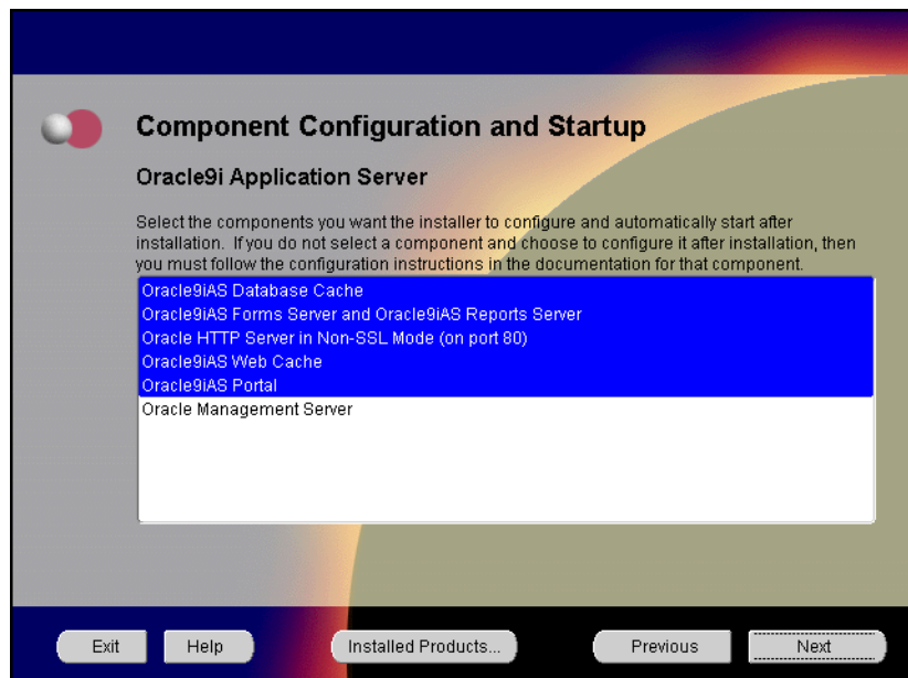
Figure 6–8 Component Configuration and Startup Screen
